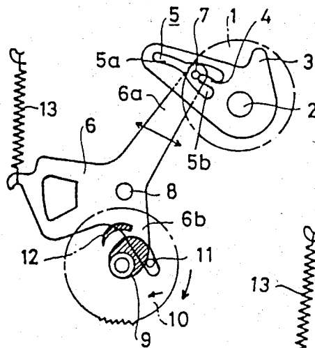
FIG. 1 PRIOR ART
