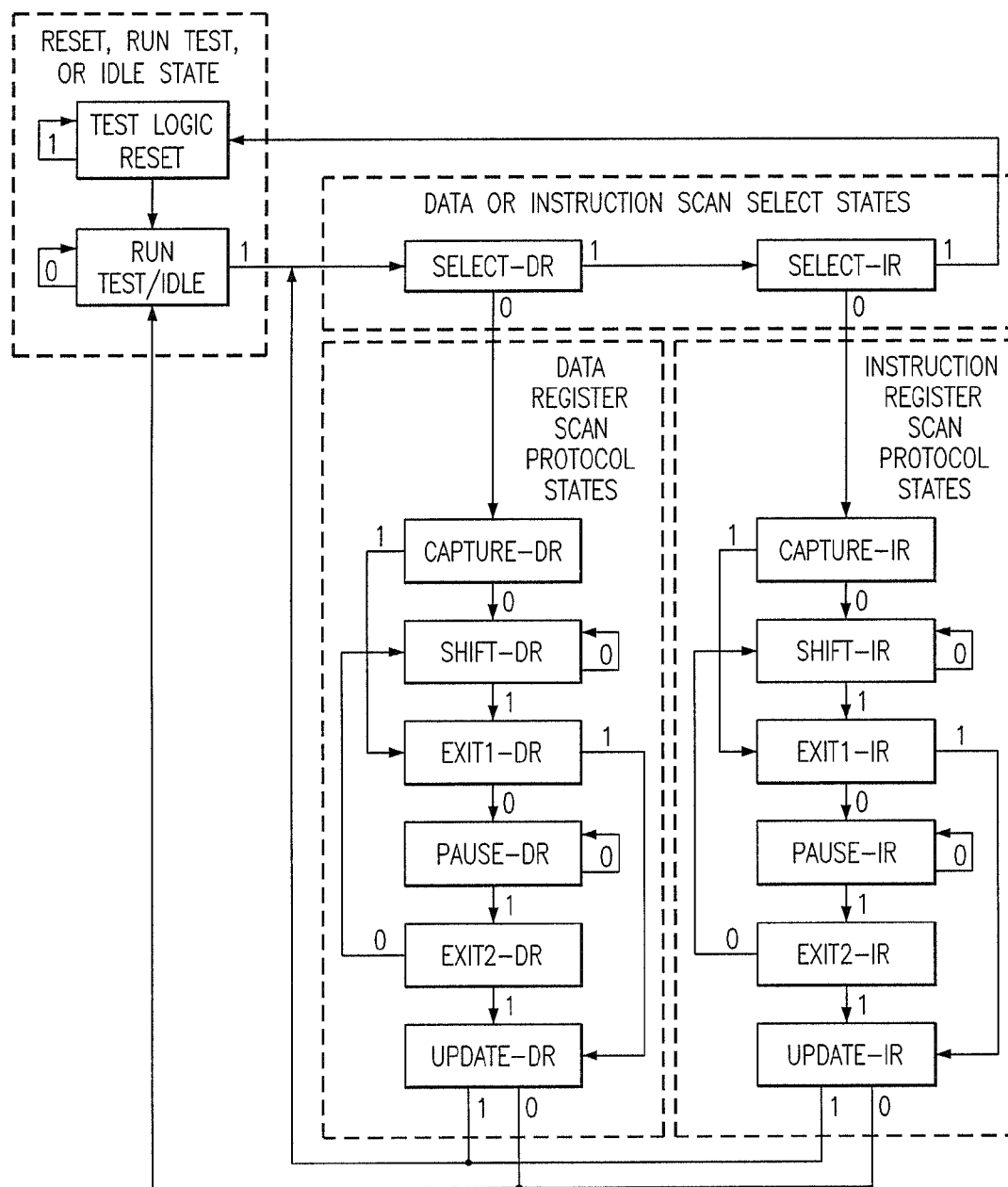
FIG. 2 (PRIOR ART)
