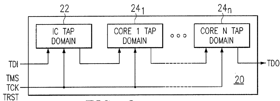
FIG. 3 (PRIOR ART)
