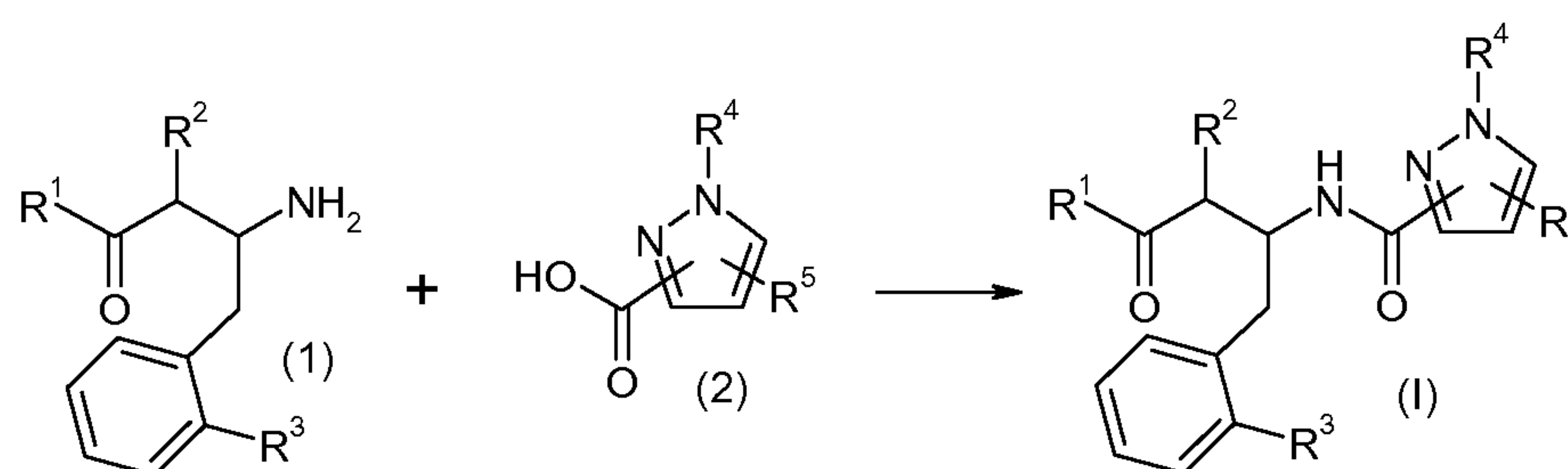
Scheme I
