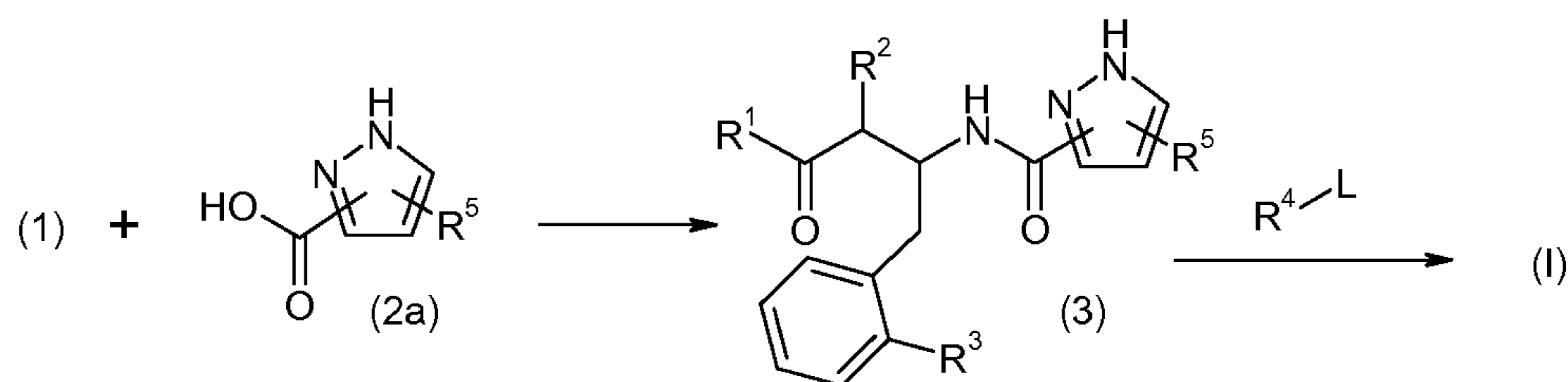
Scheme II
