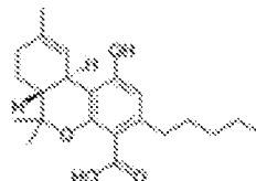
\Delta^9 -Tetrahydrocannabinolic acid B \Delta^9 -THCA-C 5 B
