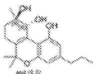
(±)-(9 R ,10 R /9 S ,10 S )- Cannabitrinol-C 3 (±)- trans -CBT-C 3
