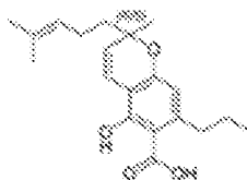
(±)-Cannabichromevarinic acid A CBCVA-C 3 A
