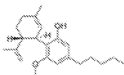
Cannabidiol monomethyl ether CBDM-C 5
