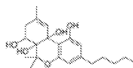
(-)-6 a ,7,10 a -Trihydroxy- Δ 9 -tetrahydrocannabinol (-)-Cannabitetrol
