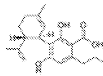
Cannabidivarinic acid CBDVA-C 3
