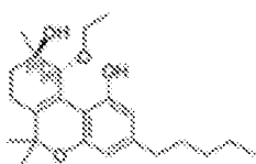
(-)-(9 R ,10 R )- trans - 10-O-Ethyl-cannabitrinol (-)- trans -CBT-OEt-C 5
