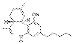
Cannabidiolic acid CBDA-C 5
