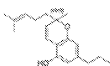
(±)-Cannabivarichromene, (±)-Cannabichromevarin CBCV-C 3
