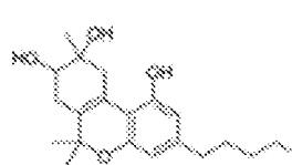
8,9-Dihydroxy-Δ 6a(10a) - tetrahydrocannabinol 8,9-Di-OH-CBT-C 5
