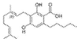
Cannabigerolic acid A ( E )-CBGA-C 5 A
