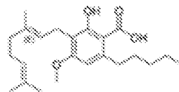
Cannabigerolic acid A monomethyl ether ( E )-CBGAM-C 5 A
