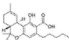
\Delta^9 -Tetrahydrocannabinolic acid A \Delta^9 -THCA-C 5 A
