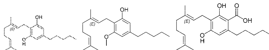
Cannabigerol monomethyl ether Cannabigerolic acid A
