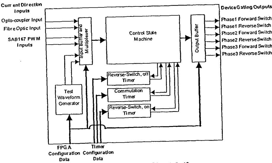
Figure 6 Schematic of the FPGA controller IC
