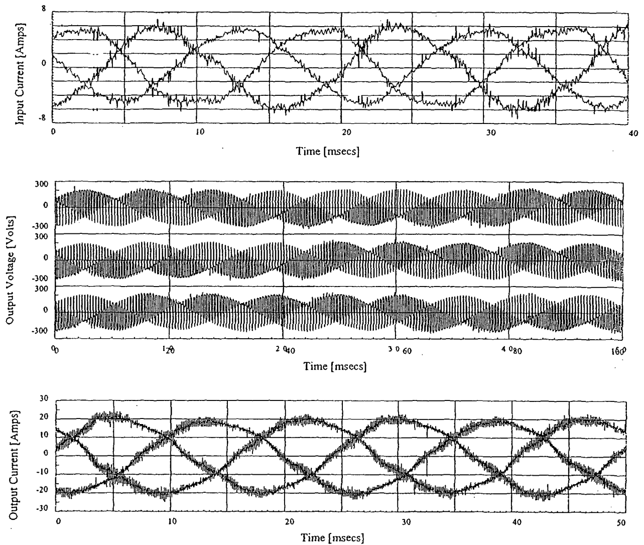
Figure 2B Input Current, Output Voltage and Output Current Waveforms for the Matrix Converter with an Induction Motor Load Switching Frequency = 4kHz, Input Frequency = 60Hz, Output frequency = 40Hz
