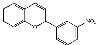
2-(3-Nitrophenyl)-2H-chromene (2l)
