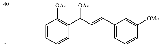
(E)-2-(1-Acetoxy-3-(3-methoxyphenyl)allyl)phenyl acetate (1f)
