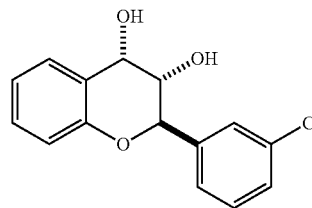
(2R,3S,4S)-2-(3-Chlorophenyl)chromane-3,4-diol (9)
