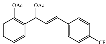
(E)-2-(1-Acetoxy-3-(4-(trifluoromethyl)phenyl)allyl)phenyl acetate (1j)
