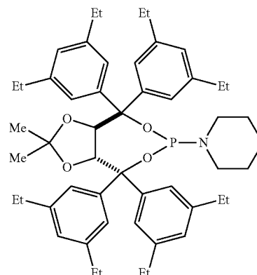
1-((3aR,8aR)-4,4,8,8-Tetrakis(3,5-diethylphenyl)-2,2-dimethyltetrahydro-[1,3]dioxolo[4,5-e][1,3,2]dioxaphosphepin-6-yl)piperidine (L3k)
