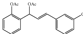
(E)-2-(1-Acetoxy-3-(3-chlorophenyl)allyl)phenyl acetate (1i)
