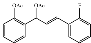
(E)-2-(1-Acetoxy-3-(2-fluorophenyl)allyl)phenyl acetate (1g)
