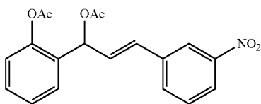
(E)-2-(1-Acetoxy-3-(3-nitrophenyl)allyl)phenyl acetate (1l)
