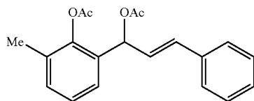
(E)-1-(2-Acetoxy-3-methylphenyl)-3-phenylallyl acetate (1p)
