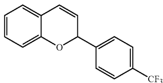
2-(4-(Trifluoromethyl)phenyl)-2H-chromene (2j)
