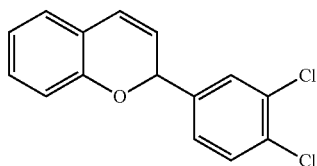
2-(3,4-Dichlorophenyl)-2H-chromene (2k)
