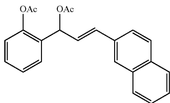
(E)-2-(1-Acetoxy-3-(naphthalen-2-yl)allyl)phenyl acetate (1c)
