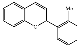
2-(o-Tolyl)-2H-chromene (2d)
