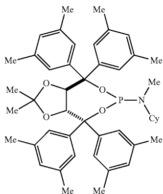
(3aR,8aR)-N-cyclohexyl-4,4,8,8-tetrakis(3,5-dimethylphenyl)-N,2,2-trimethyltetrahydro-[1,3]dioxolo[4,5-e][1,3,2]dioxaphosphepin-6-amine (L3j)
