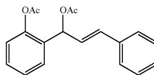
(E)-1-(2-Acetoxy-3-methylphenyl)-3-phenylallyl acetate (1a)
