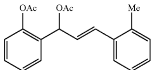
(E)-2-(1-Acetoxy-3-(o-tolyl)allyl)phenyl acetate (1d)
