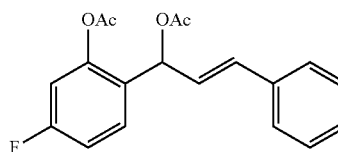
(E)-2-(1-Acetoxy-3-phenylallyl)-5-fluorophenyl acetate (1m)
