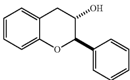
(2R,3S)-2-Phenylchroman-3-ol (7)
