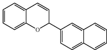
2-(Naphthalen-2-yl)-2H-chromene (2c)
