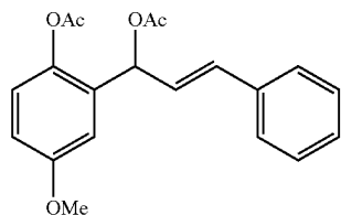
(E)-2-(1-Acetoxy-3-phenylallyl)-4-methoxyphenyl acetate (1o)
