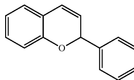
2-Phenyl-2H-chromene (2a)
