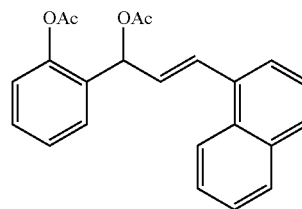
(E)-2-(1-Acetoxy-3-(naphthalen-1-yl)allyl)phenyl acetate (1b)
