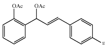
(E)-2-(1-Acetoxy-3-(4-fluorophenyl)allyl)phenyl acetate (1h)
