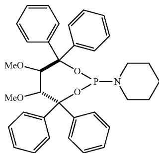
1-((5R,6R)-5,6-Dimethoxy-4,4,7,7-tetraphenyl-1,3,2-dioxaphosphhepan-2-yl)piperidine (L4)
