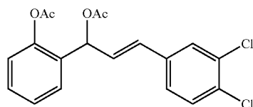
(E)-2-(1-Acetoxy-3-(3,4-dichlorophenyl)allyl)phenyl acetate (1k)
