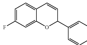
7-Fluoro-2-phenyl-2H-chromene (2m)
