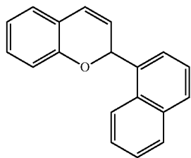
2-(Naphthalen-1-yl)-2H-chromene (2b)
