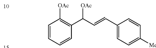
(E)-2-(1-Acetoxy-3-(p-tolyl)allyl)phenyl acetate (1e)
