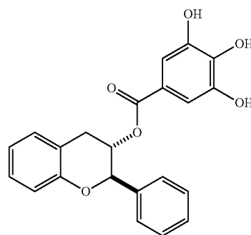
(2R,3S)-2-Phenylchroman-3-yl 3,4,5-trihydroxybenzoate (8)
