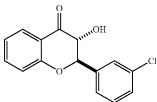
(2R,3R)-2-(3-chlorophenyl)-3-hydroxychroman-4-one (10)
