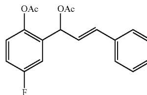
(E)-2-(1-Acetoxy-3-phenylallyl)-4-fluorophenyl acetate (1n)
