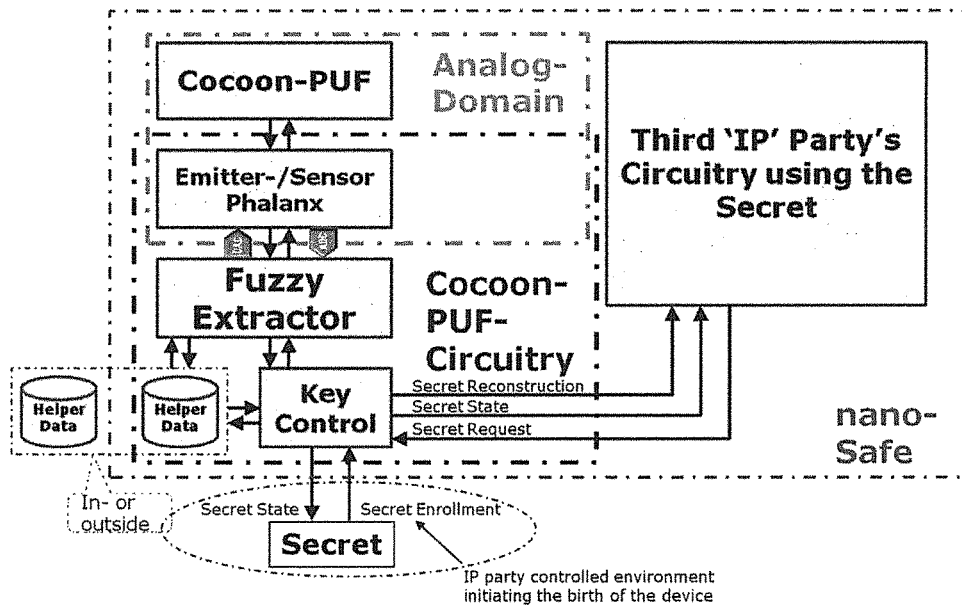
Figure 21: Block Diagram of a CASTOR.
