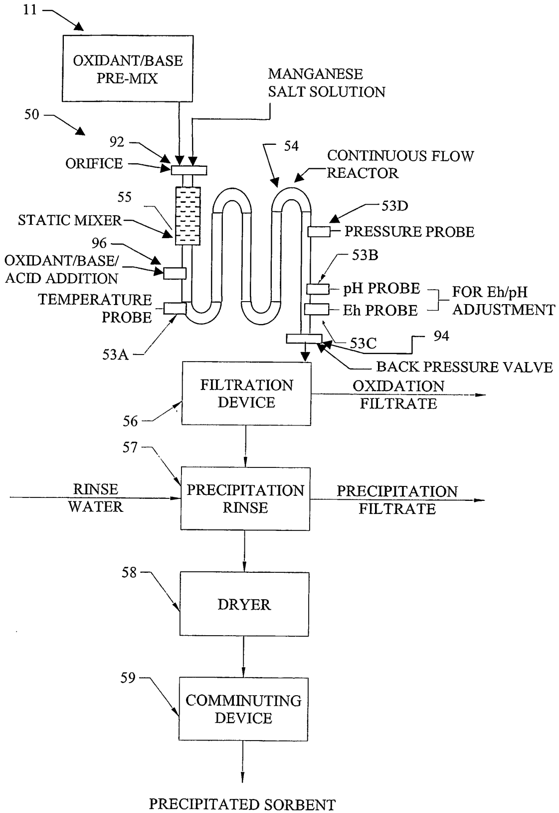
FIGURE 7 PRECIPITATION OF VIRGIN OXIDES OF MANGANESE SORBENT
