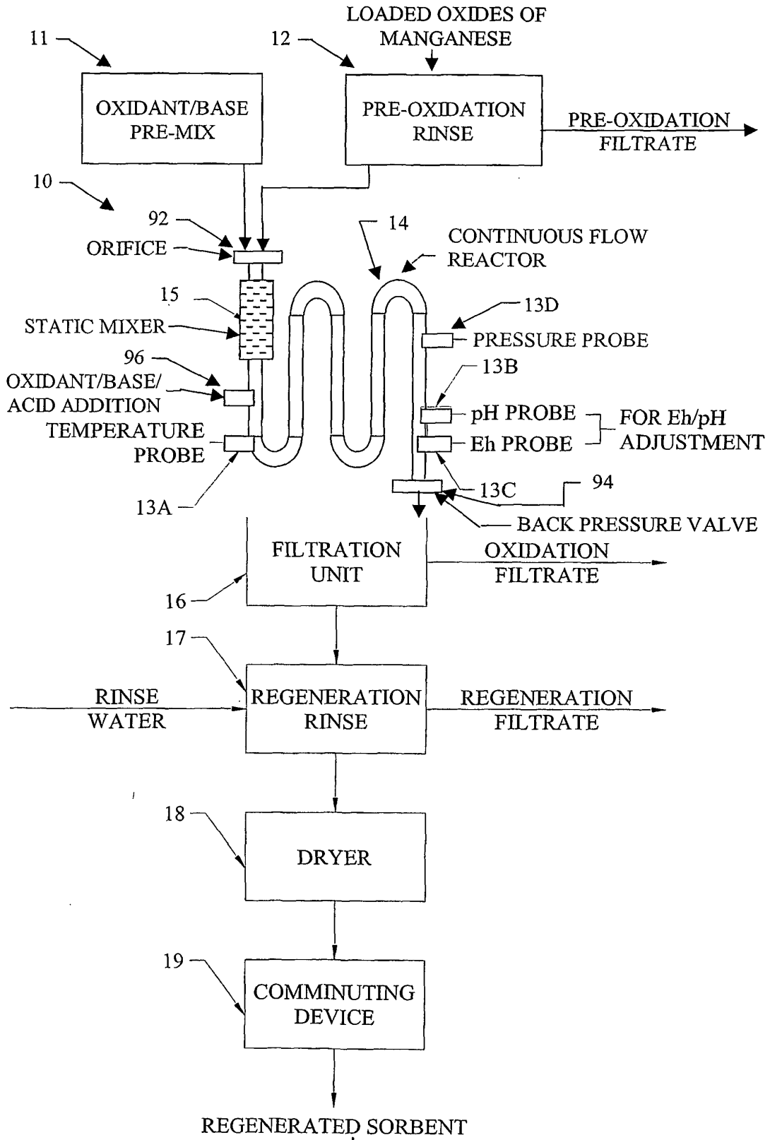
FIGURE 3 REGENERATION OF LOADED SORBENT
