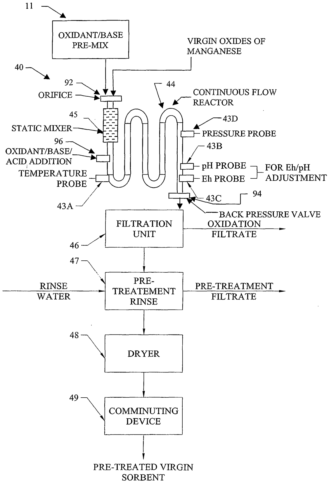
FIGURE 6 PRE-TREATMENT OF VIRGIN SORBENT
