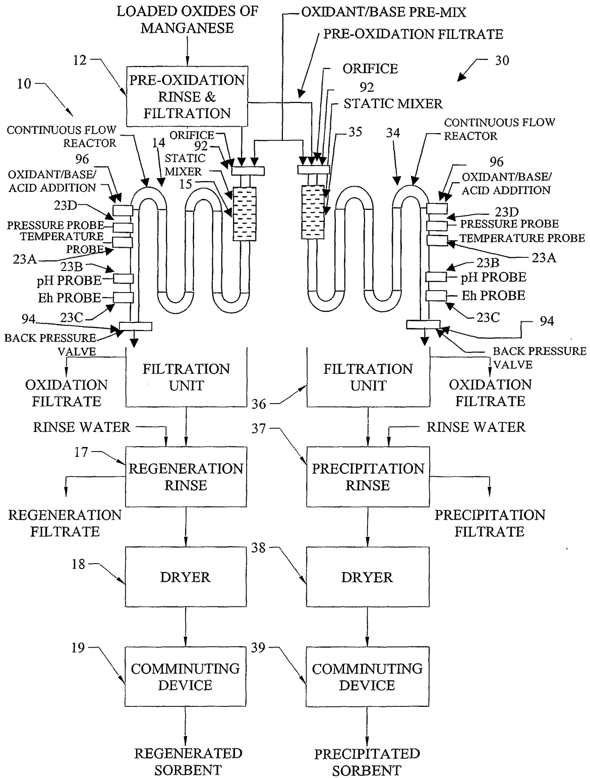
FIGURE 5 REGENERATION & PRECIPITATION OF SORBENT
