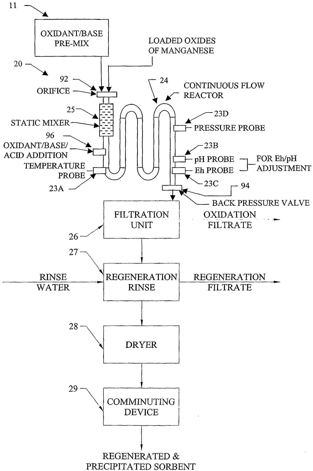
FIGURE 4 REGENERATION OF LOADED SORBENT
