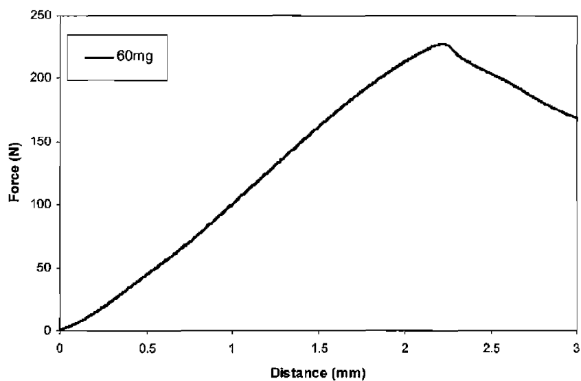
Example 20 Indentation Test of Example 16.1 tablet
