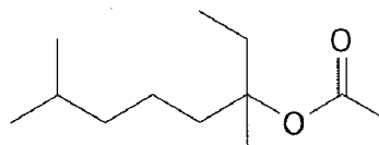
Tetrahydrolinalyl acetate
