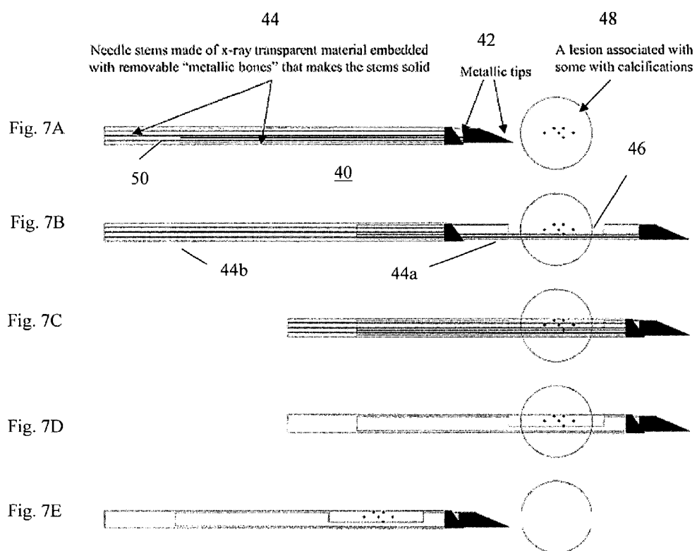
Figure 7 Illustration of biopsy needle with two radio-opaque tips and transparent body embedded with metallic stiffening rods
