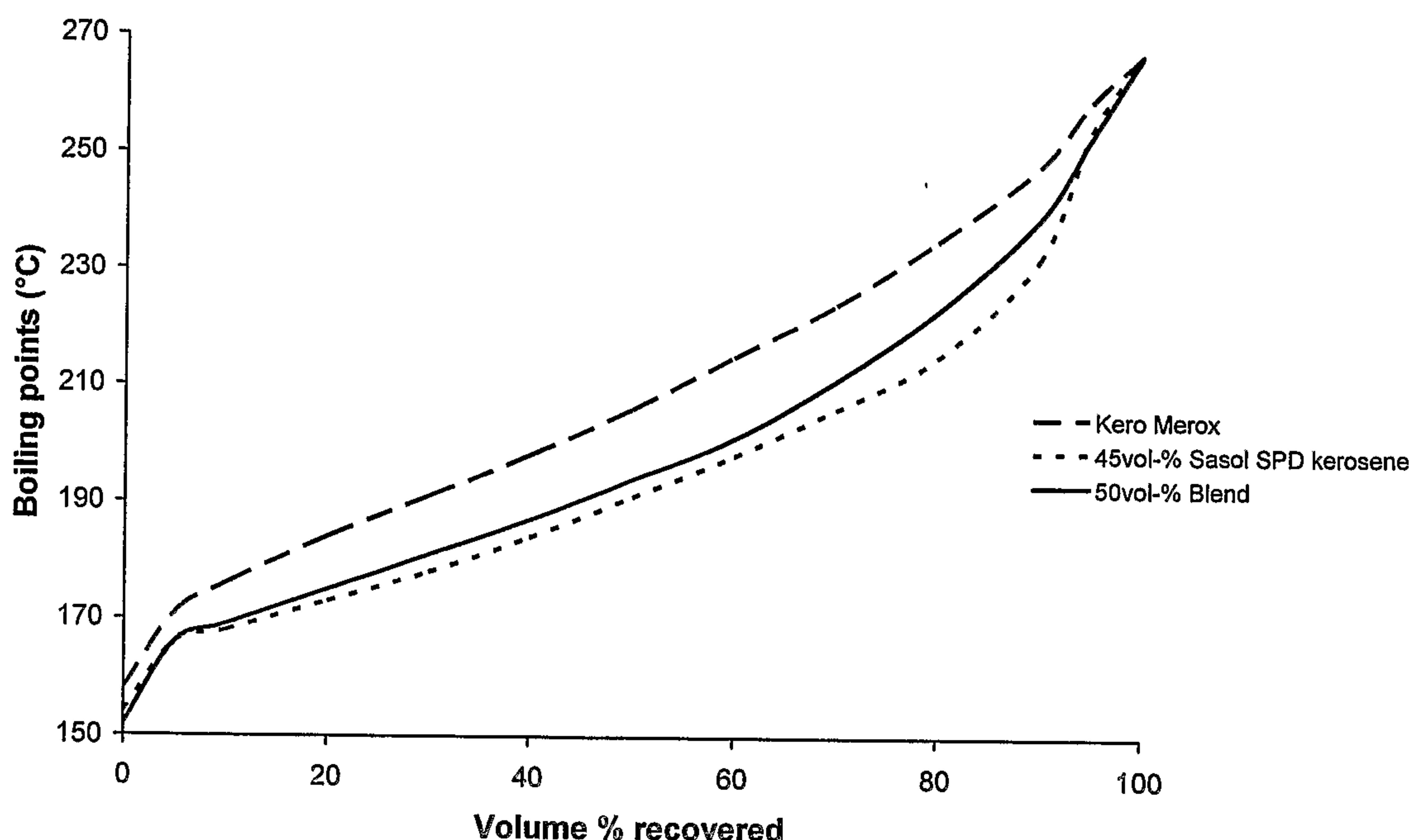
Figure 11: Distillation profiles of sweetened Kero Merox™ kerosene, the 45% Sasol SPD™ kerosene fraction and a 50% blend thereof
