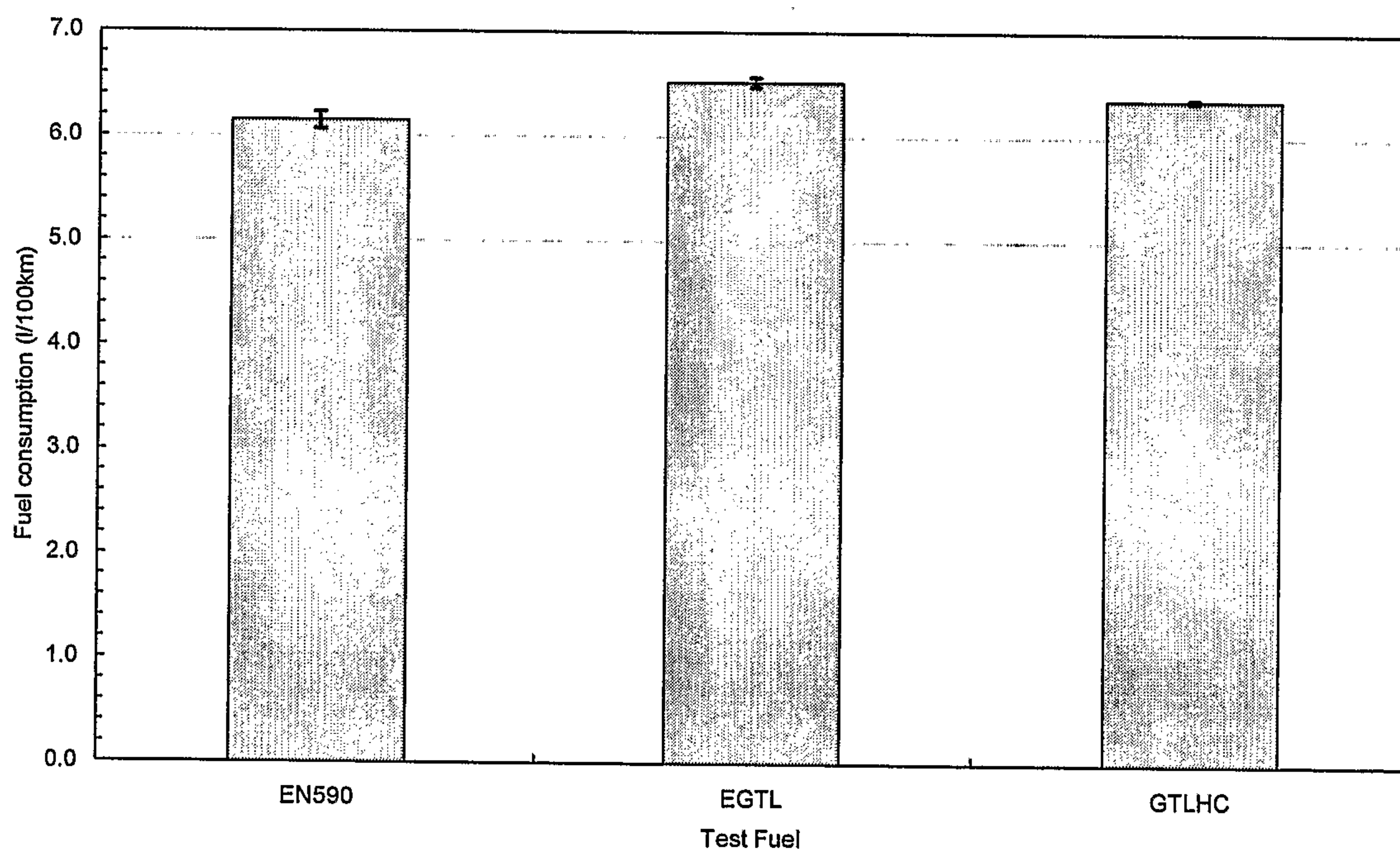
Figure 8 : Fuel Consumption
