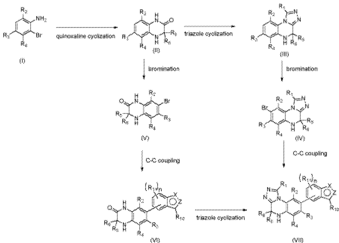
Reaction scheme 1:
