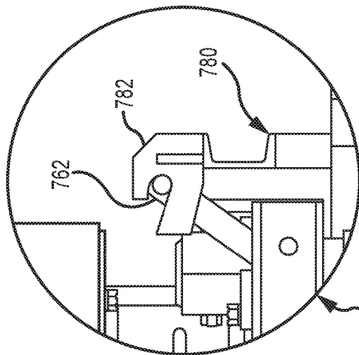
DETAIL C FIG. 27
