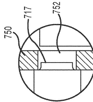
DETAIL D FIG. 28
