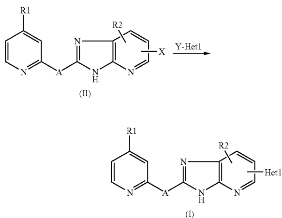
Reaction Scheme 1:
