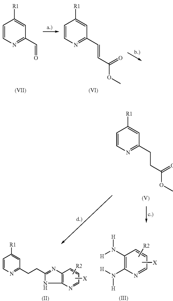
Reaction Scheme 2:
