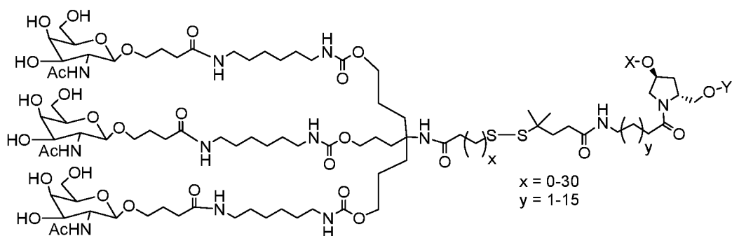
MONOMER 3
