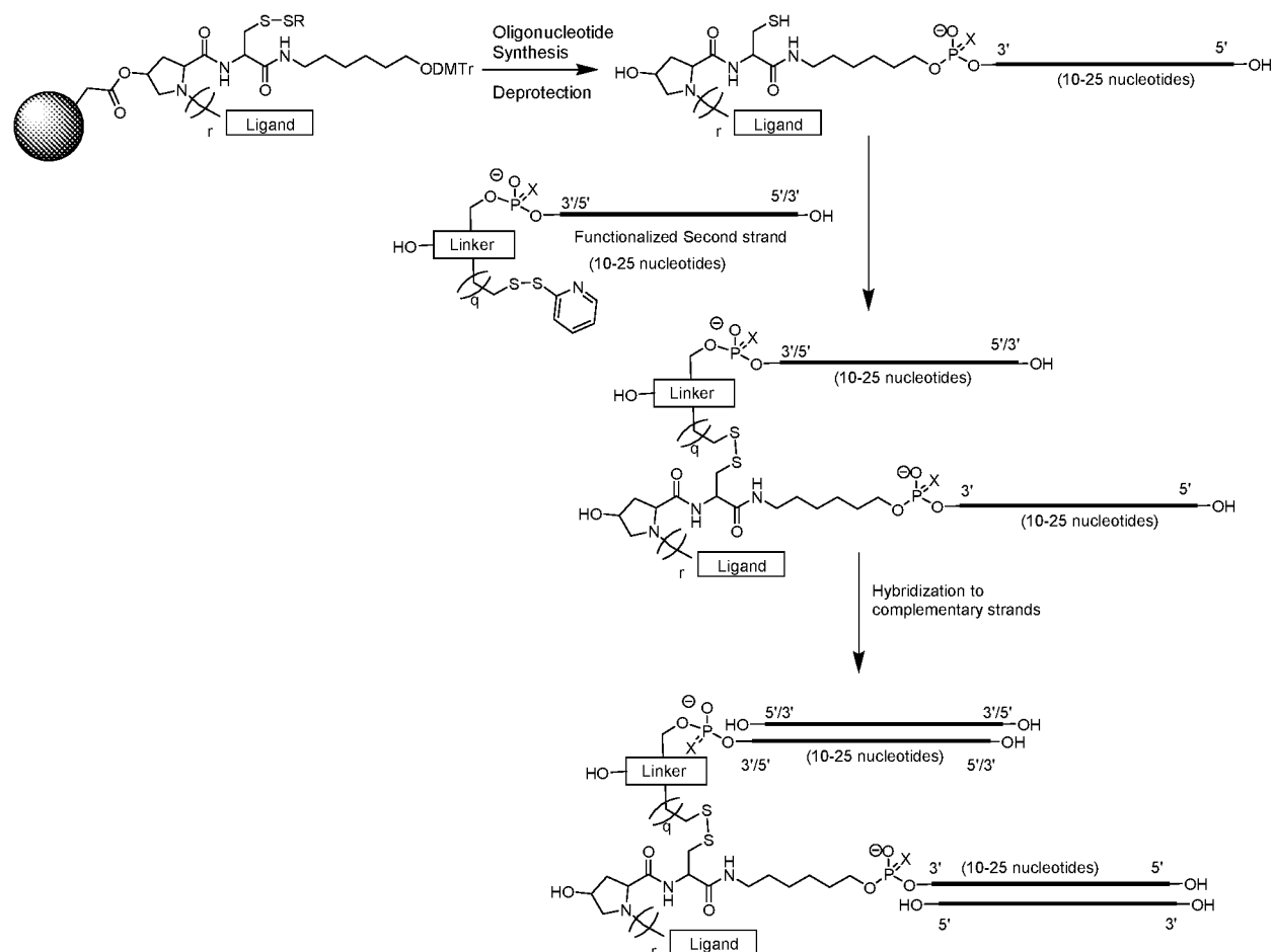
Scheme 6.
