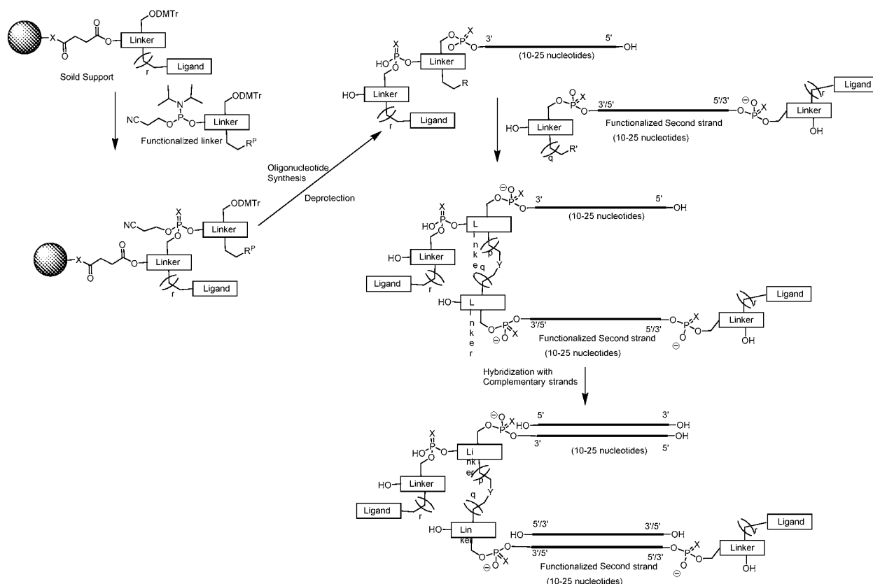
Scheme 4.
