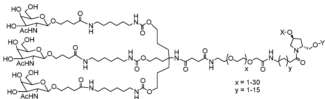
MONOMER 2.
