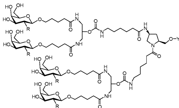
MONOMER 24
