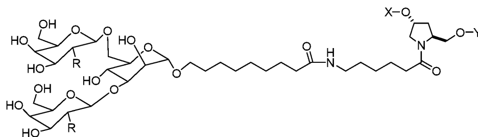
MONOMER 28
