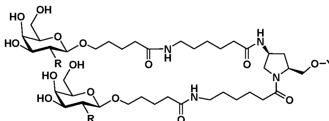
MONOMER 22
