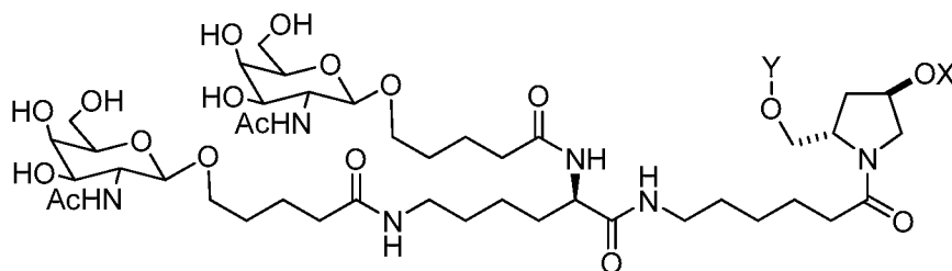
MONOMER 12
