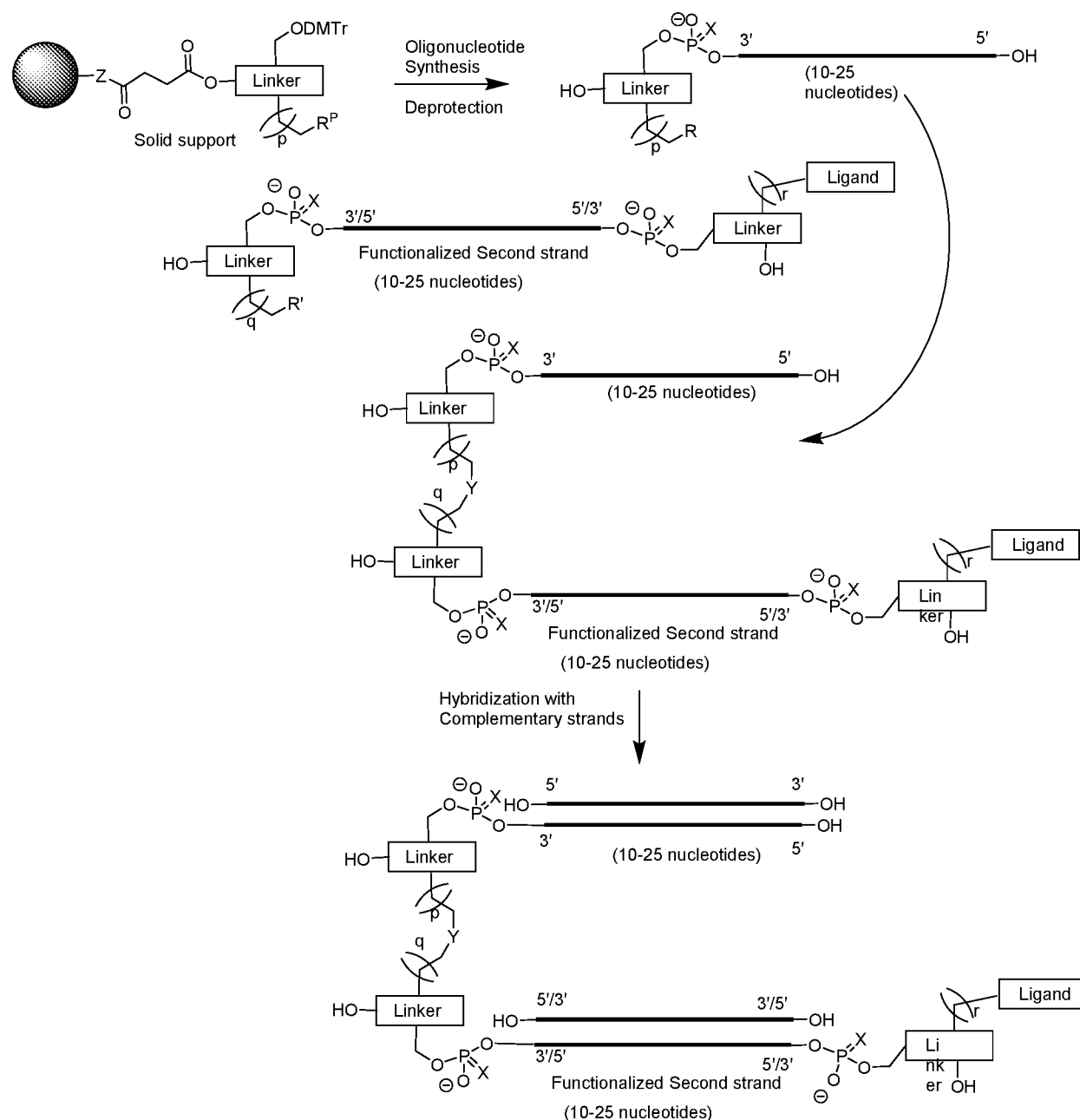
Scheme 2.
