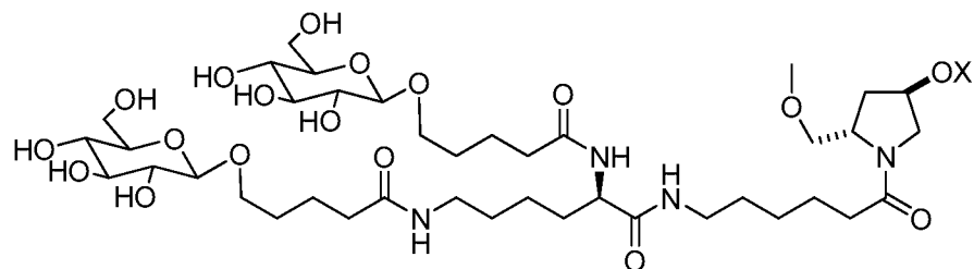
MONOMER 11
