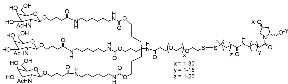
MONOMER 6.
