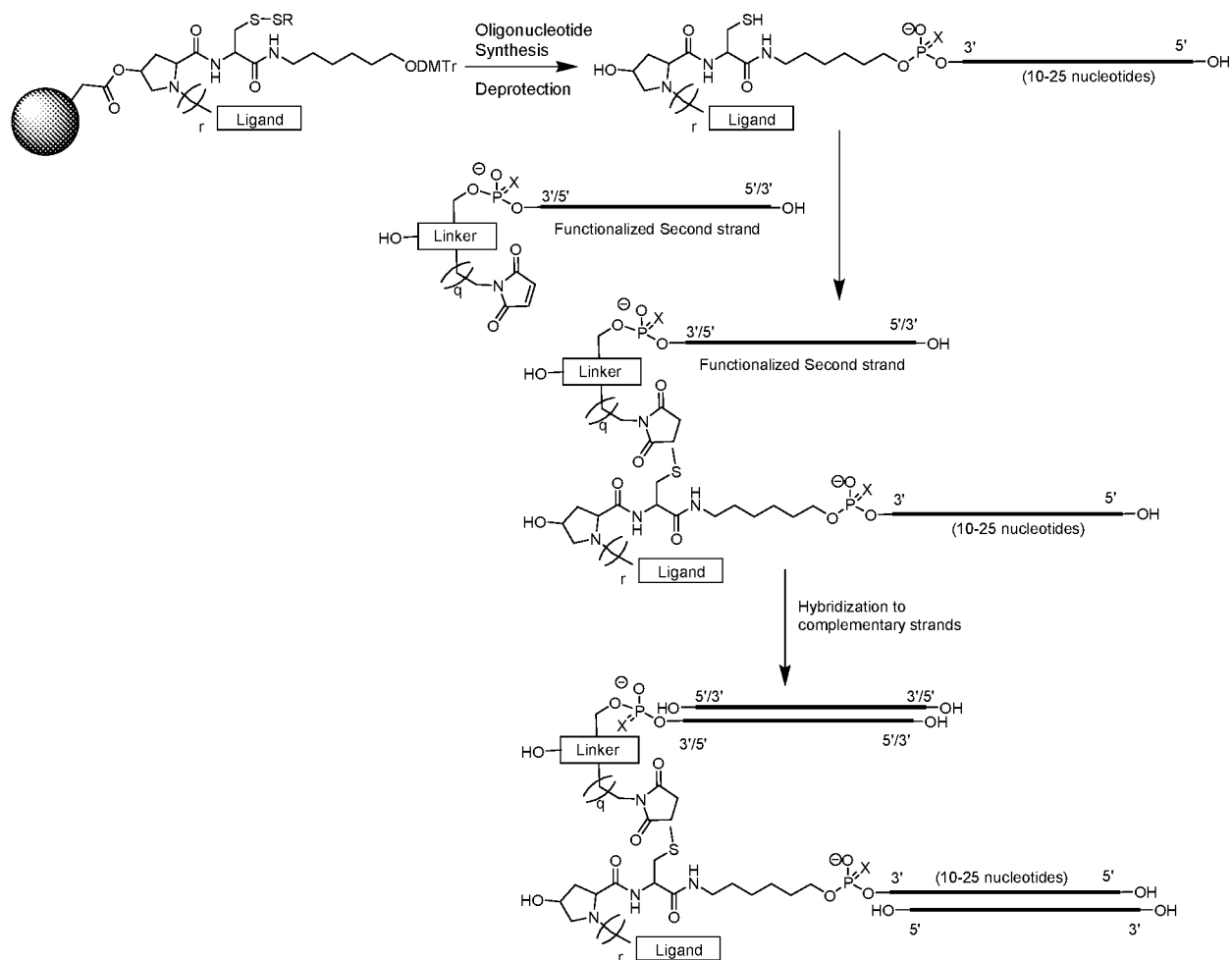
Scheme 7.
