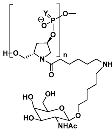
MONOMER 18
