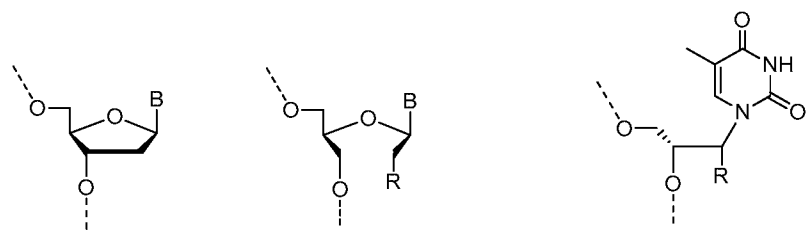
unlocked nucleic acid R= H, OH, O-alkyl
