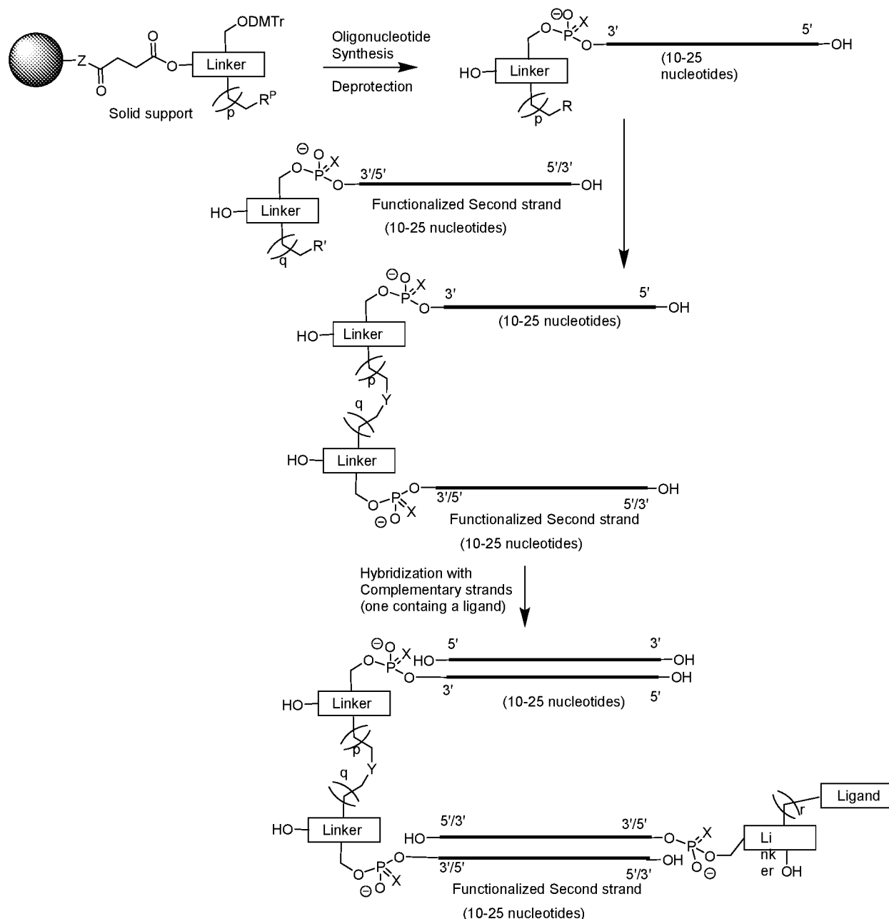
Scheme 5.
