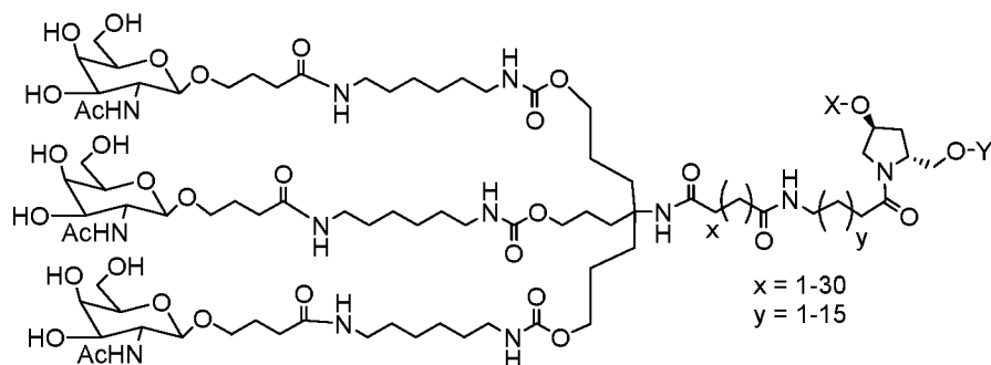
MONOMER 1.
