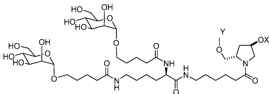
MONOMER 10
