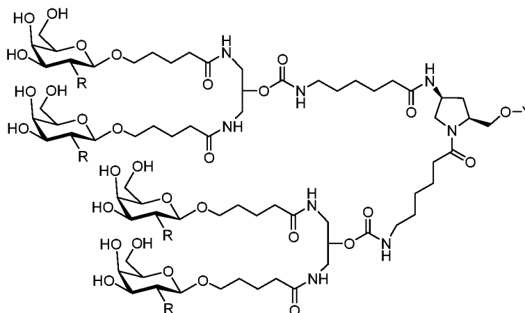
MONOMER 21
