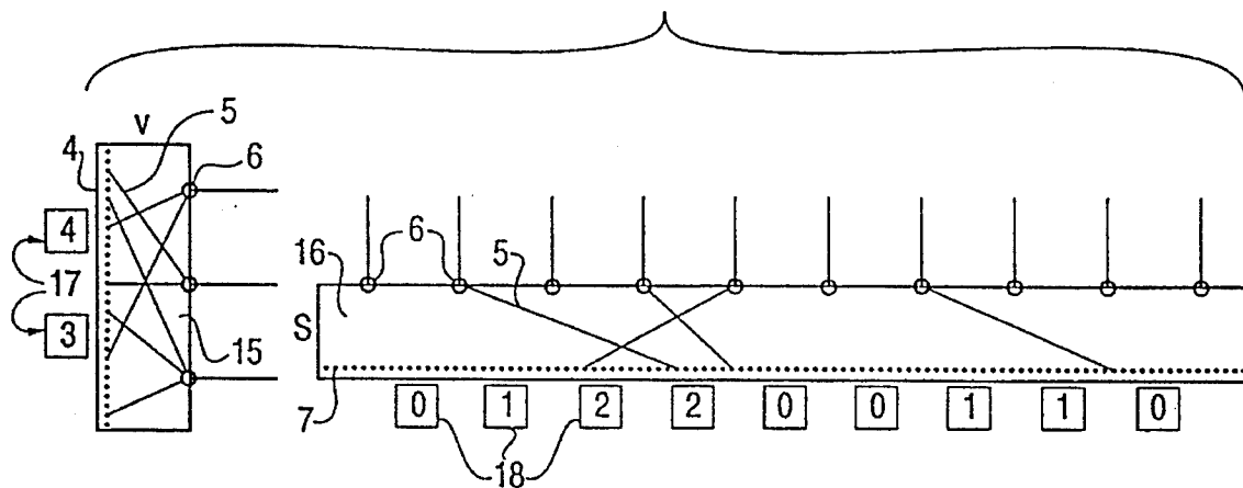
FIG. 3 PRIOR ART
