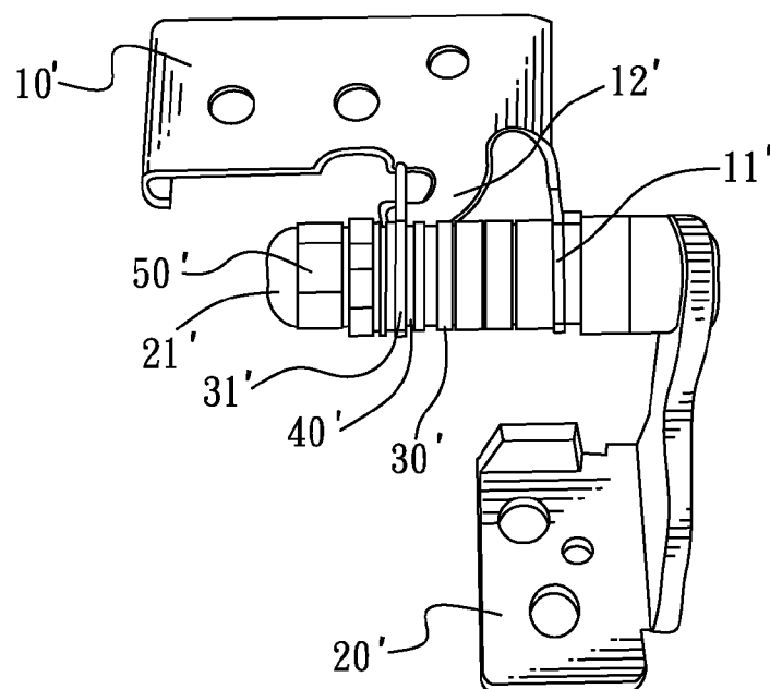
FIG. 7 (Prior Art)
