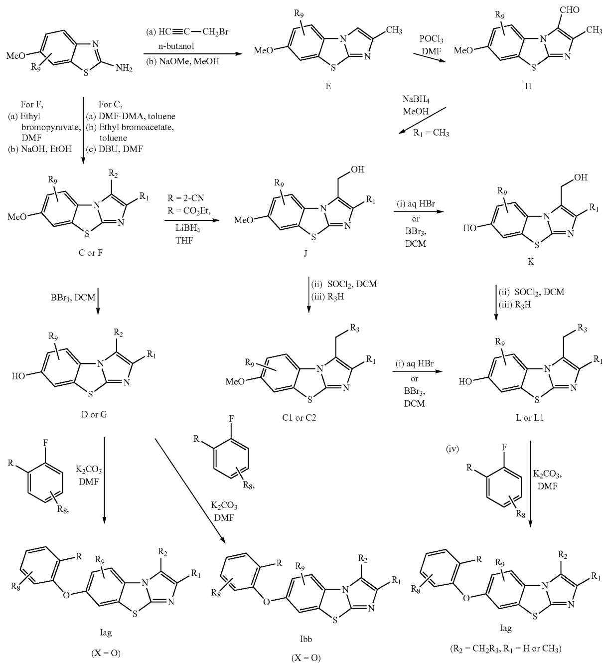
Scheme - 5
