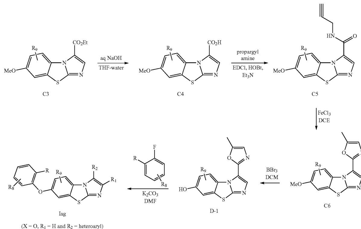
Scheme - 5a
