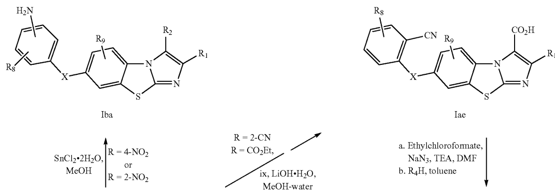
Scheme - 4
