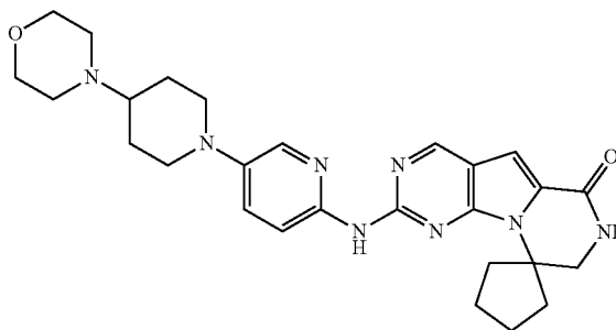
Compound 39
