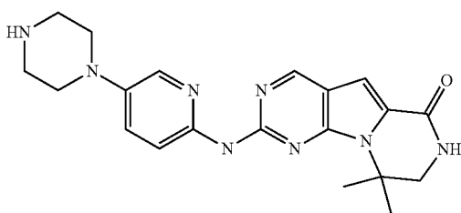
Compound 26
