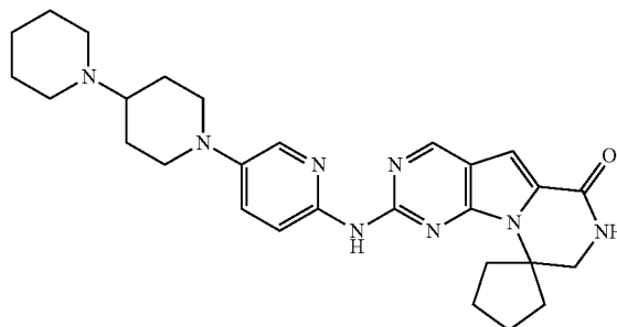
Compound 40
