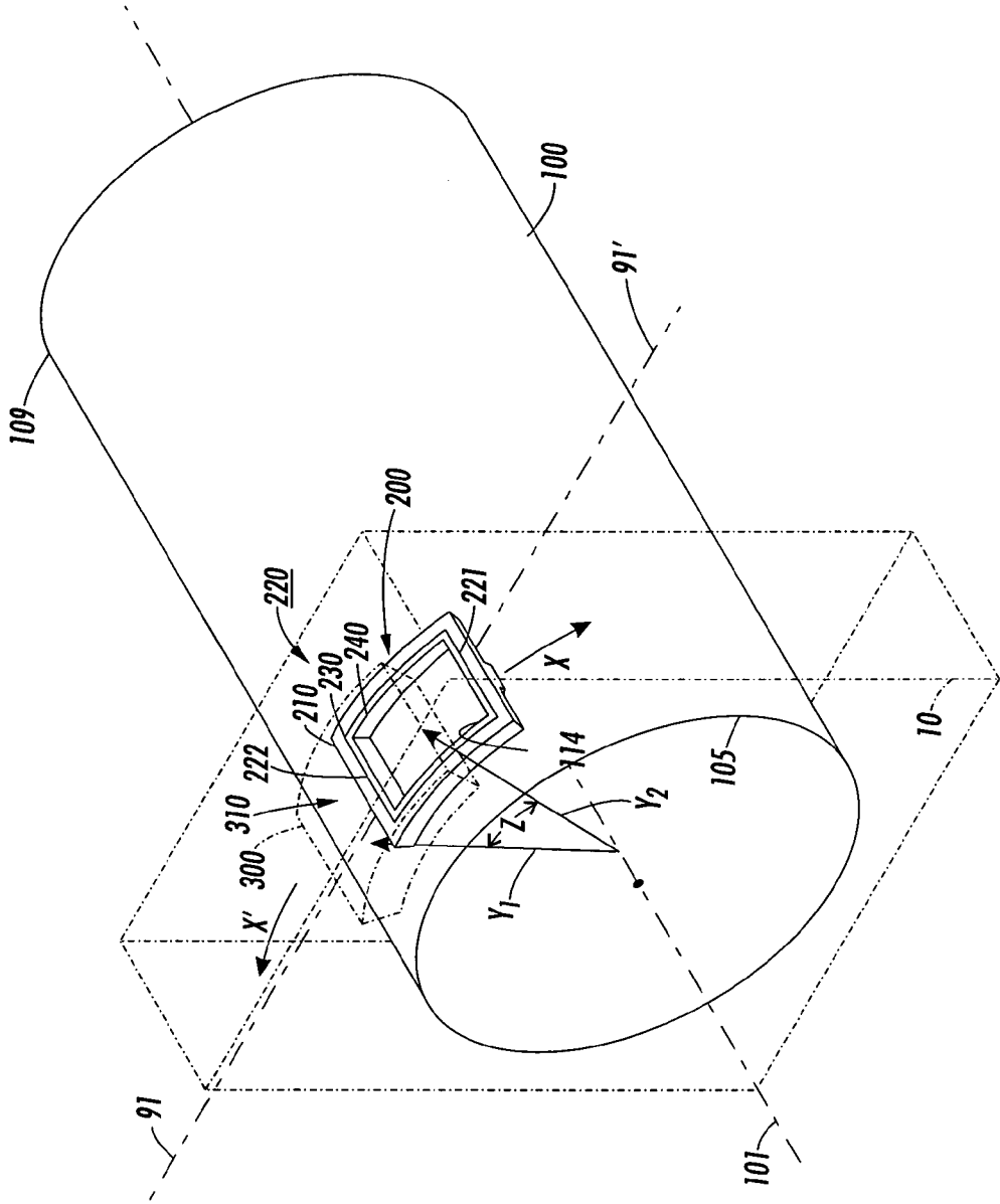
FIG. 2 PRIOR ART
