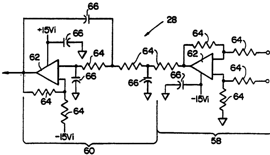
FIG. 3. PRIOR ART
