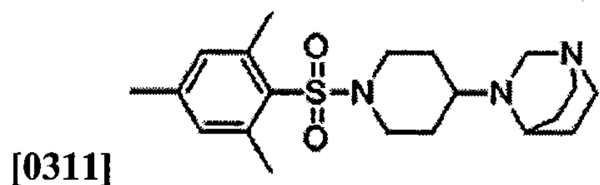
3-(4-(mesitylsulfonyl)piperazin-1-yl)quinuclidine:
