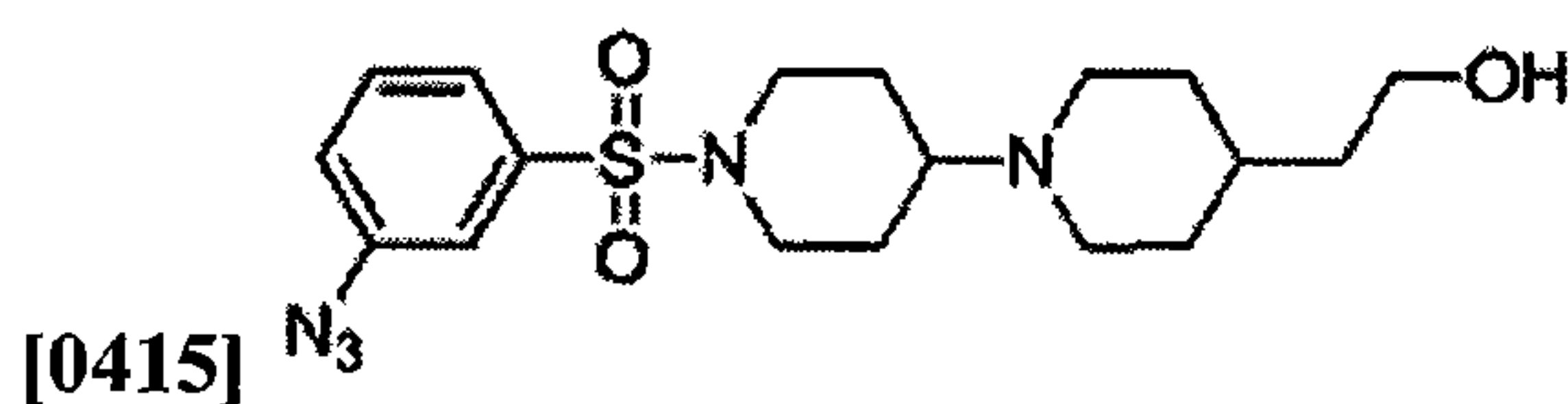
2-(1'-((3-azidophenyl)sulfonyl)-[1,4'-
