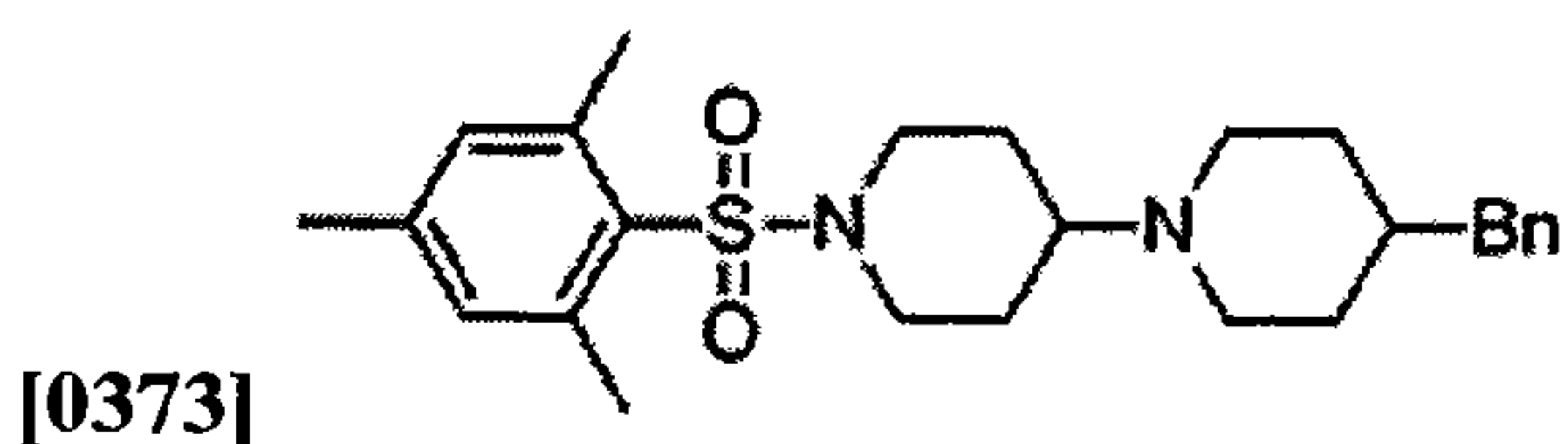
4-benzyl-1'-(mesitylsulfonyl)-1,4'-bipiperidine:
