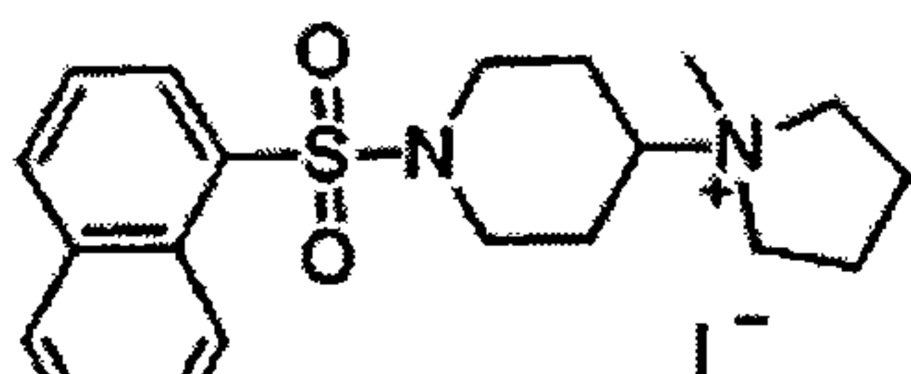
[0358] 1-methyl-1-(1-(naphthalen-1-ylsulfonyl)piperidin-4-yl)pyrrolidin-1-ium iodide:
