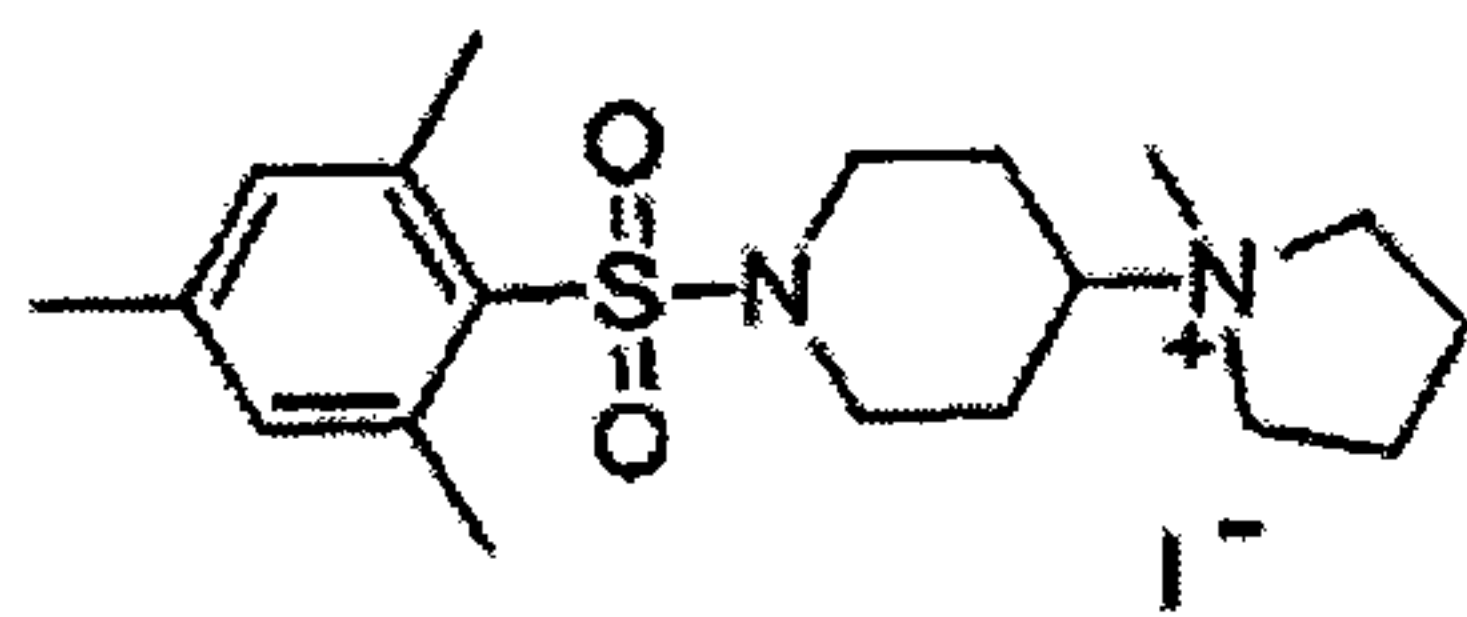
[0357] 1-(1-(mesitylsulfonyl)piperidin-4-yl)-1-methylpyrrolidin-1-ium iodide:
