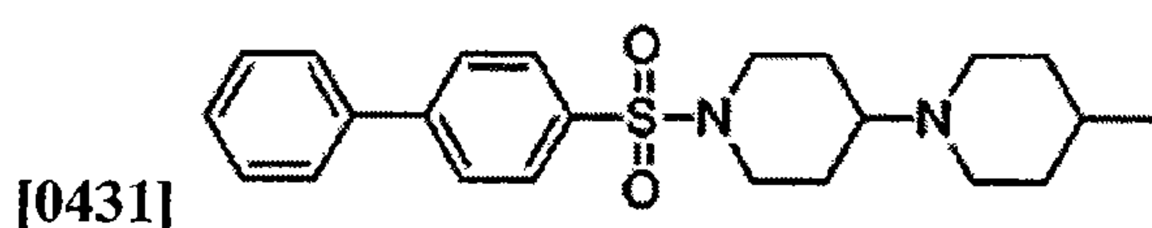
1'-([1,1'-biphenyl]-4-ylsulfonyl)-4-methyl-
