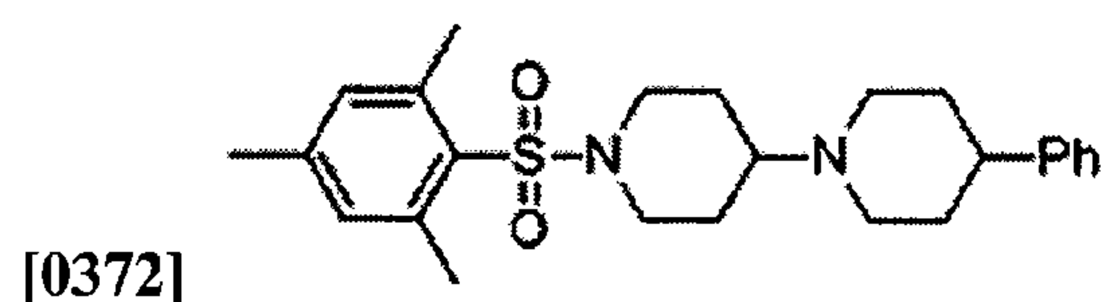
1'-(mesitylsulfonyl)-4-phenyl-1,4'-bipiperidine:
