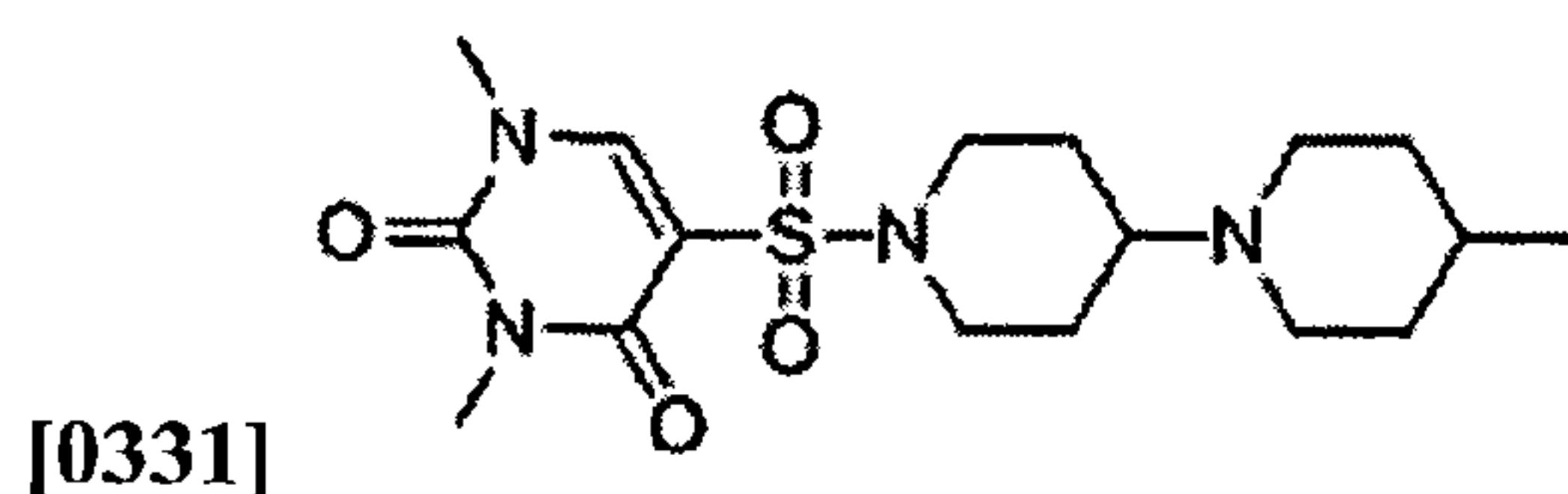
1,3-dimethyl-5-((4-methyl-[1,4'-bipiperidin]-1'-
