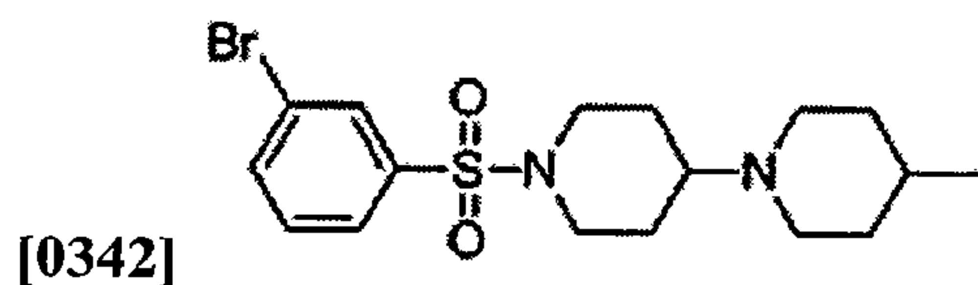
1'-((3-bromophenyl)sulfonyl)-4-methyl-1,4'-
