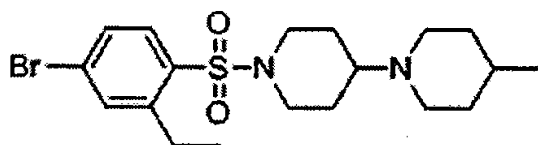
[0317] 1'-((4-bromo-2-ethylphenyl)sulfonyl)-4-methyl-1,4'-bipiperidine:
