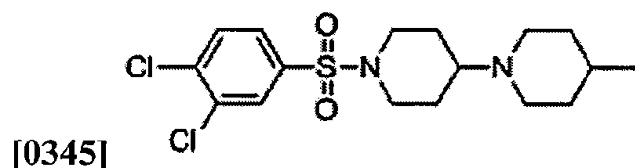
1'-((3,4-dichlorophenyl)sulfonyl)-4-methyl-1,4'-
