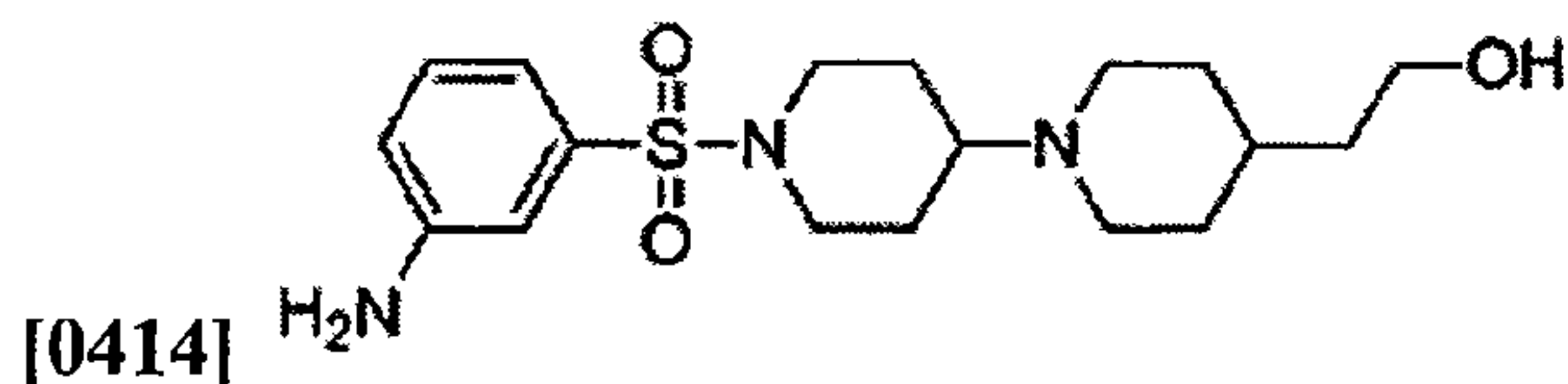
2-(1'-((3-aminophenyl)sulfonyl)-[1,4'-
