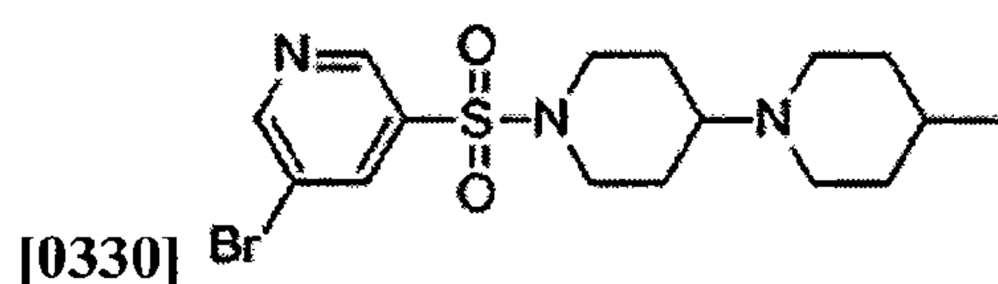
1'-((5-bromopyridin-3-yl)sulfonyl)-4-methyl-1,4'-
