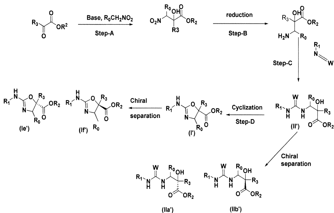
Scheme 2
