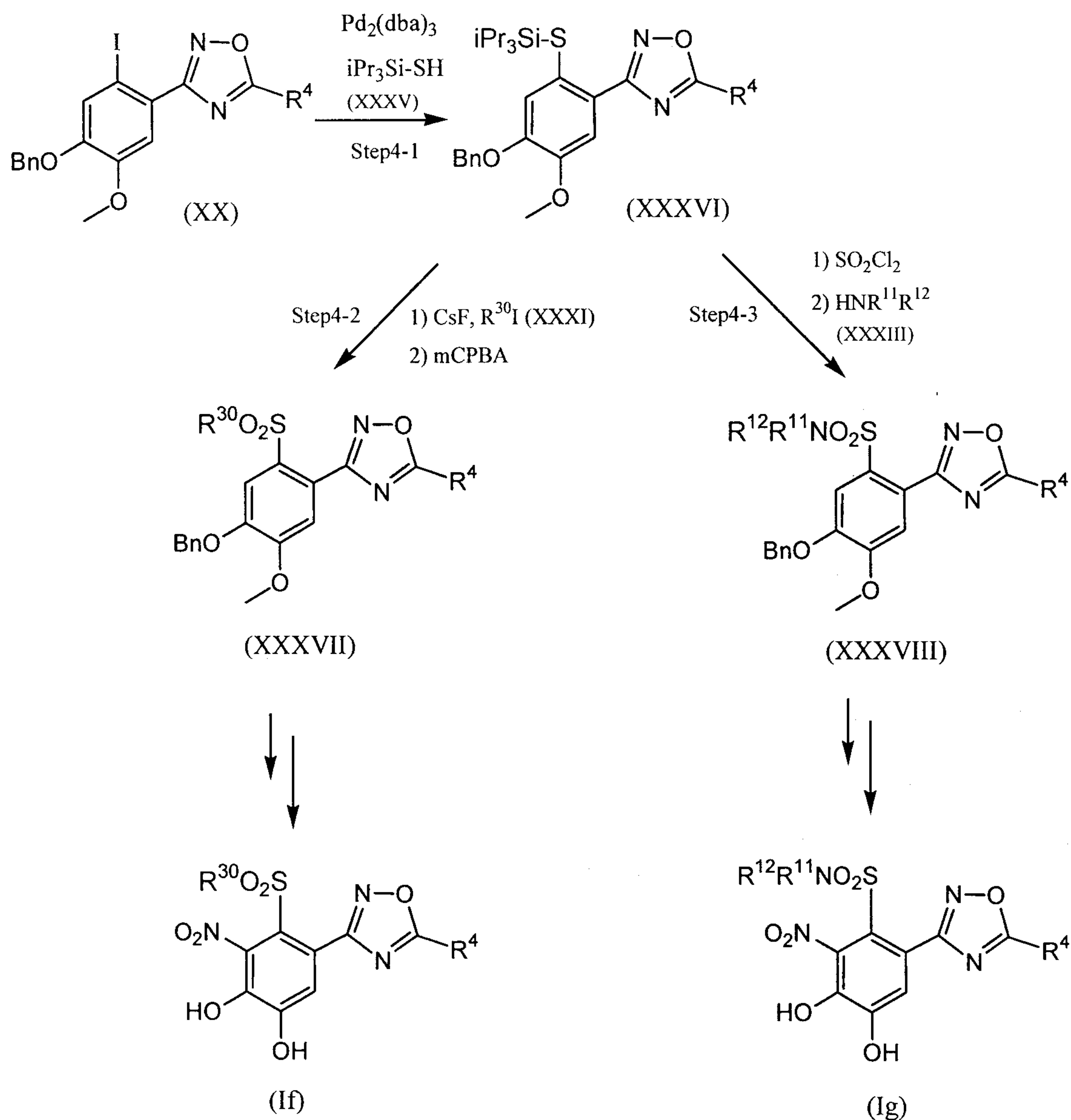
Scheme 4
