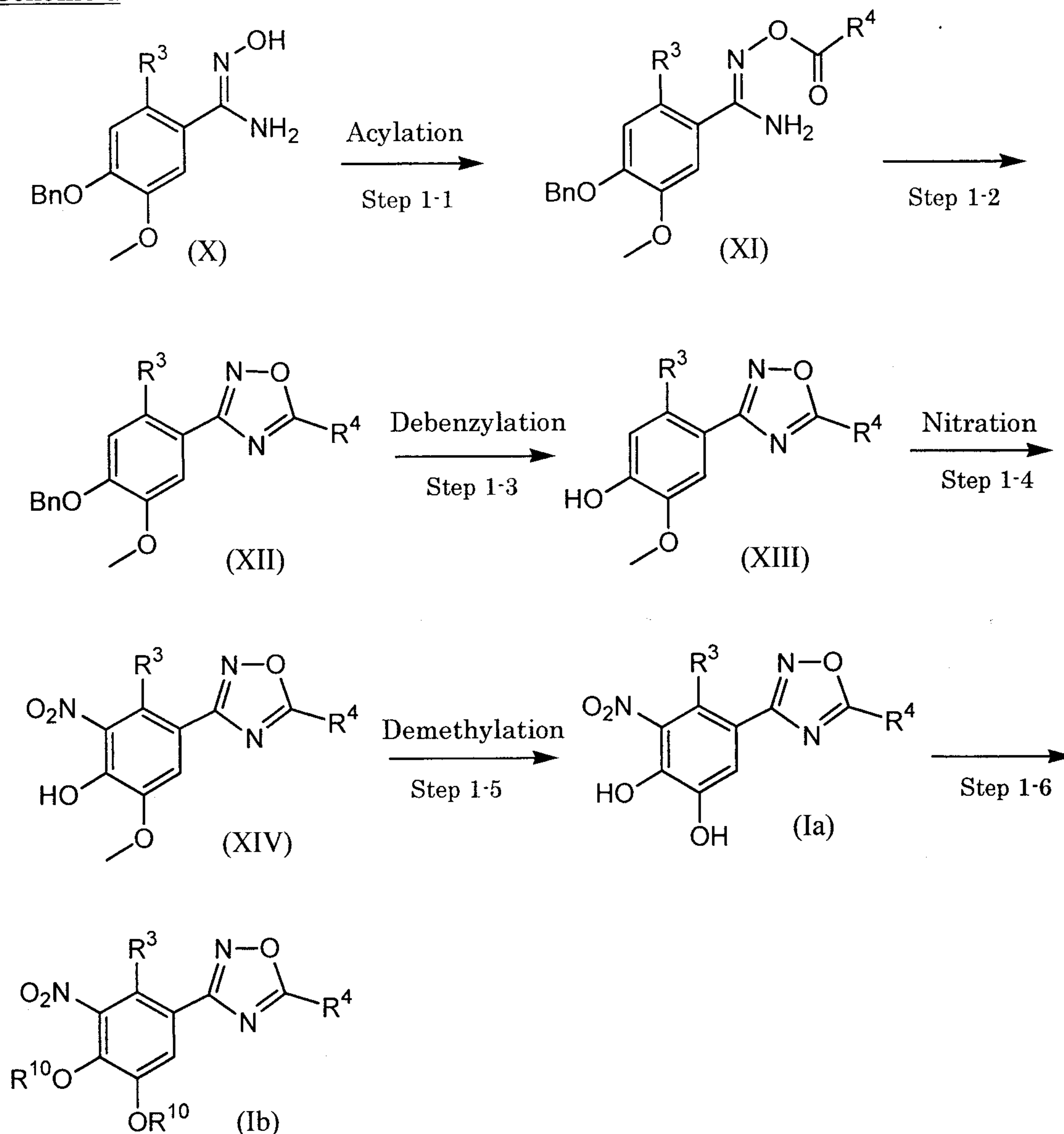
Scheme 1
