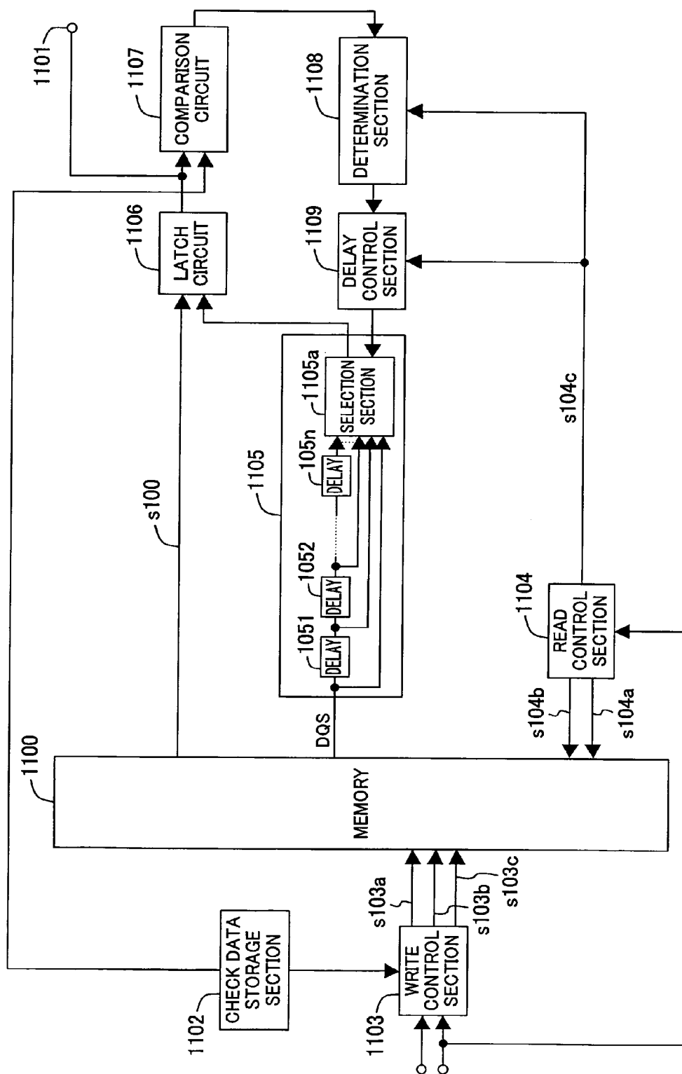
FIG. 13 PRIOR ART
