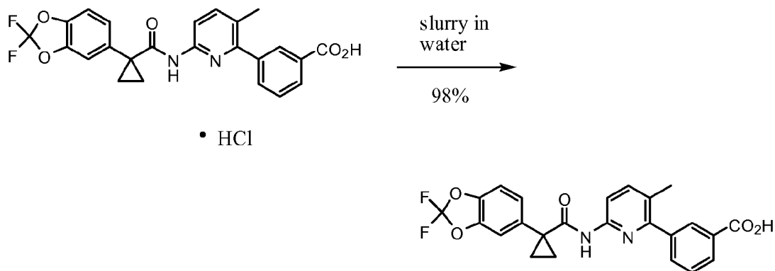
40 Compound 1
