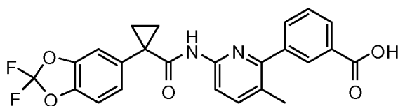
Compound 1
