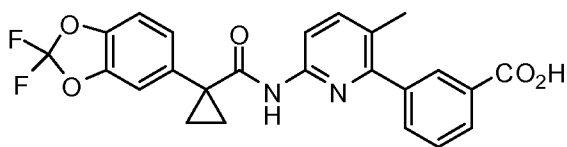
Compound 1.
