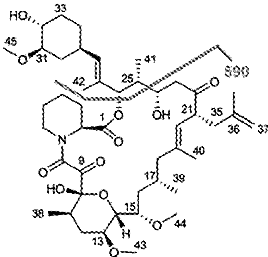
36-Methyl-FK506
