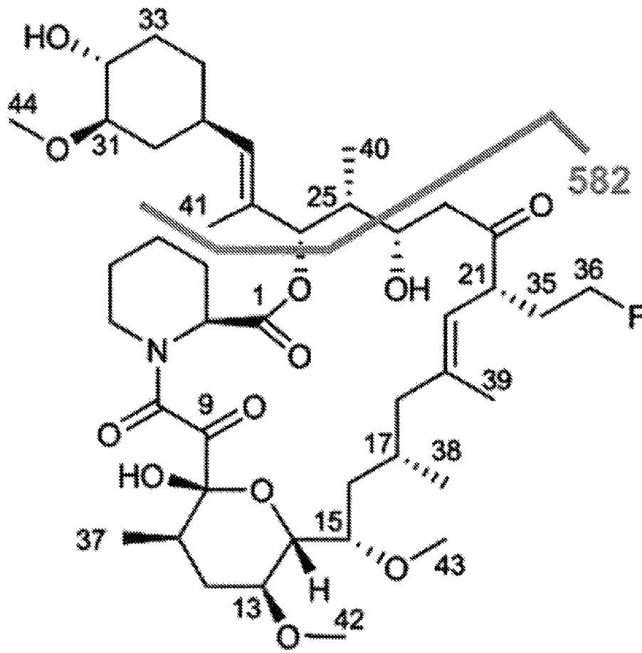
36-Fluoro-FK520
