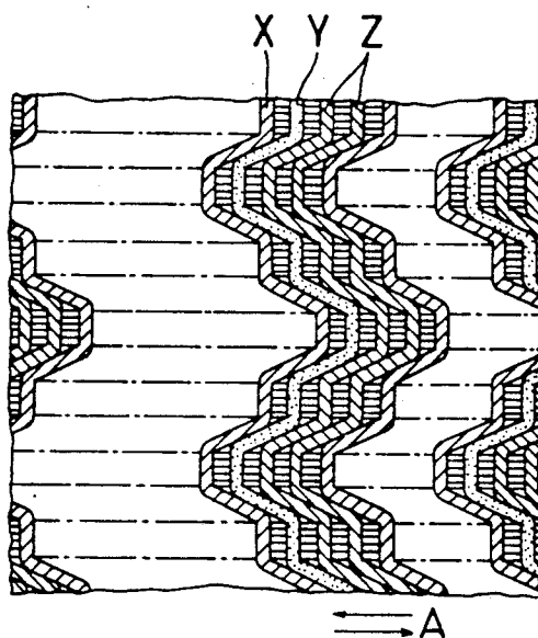
PRIOR ART FIG. 10
