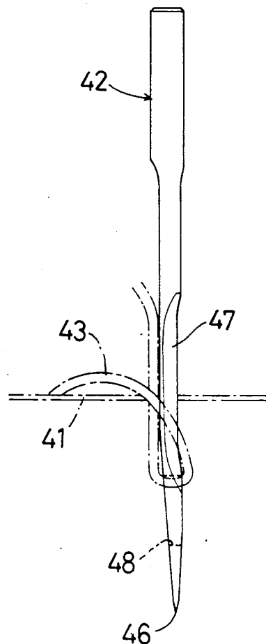
PRIOR ART FIG. 12
