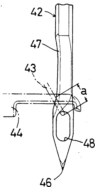
PRIOR ART FIG. 11
