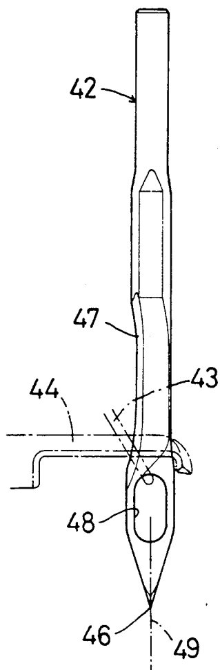
PRIOR ART FIG. 9
