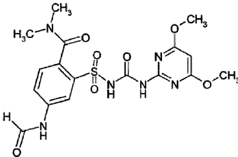
(chemical formula of foramsulfuron)
