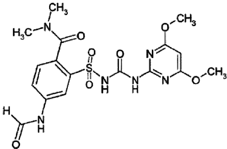
(chemical formula of foramsulfuron)
