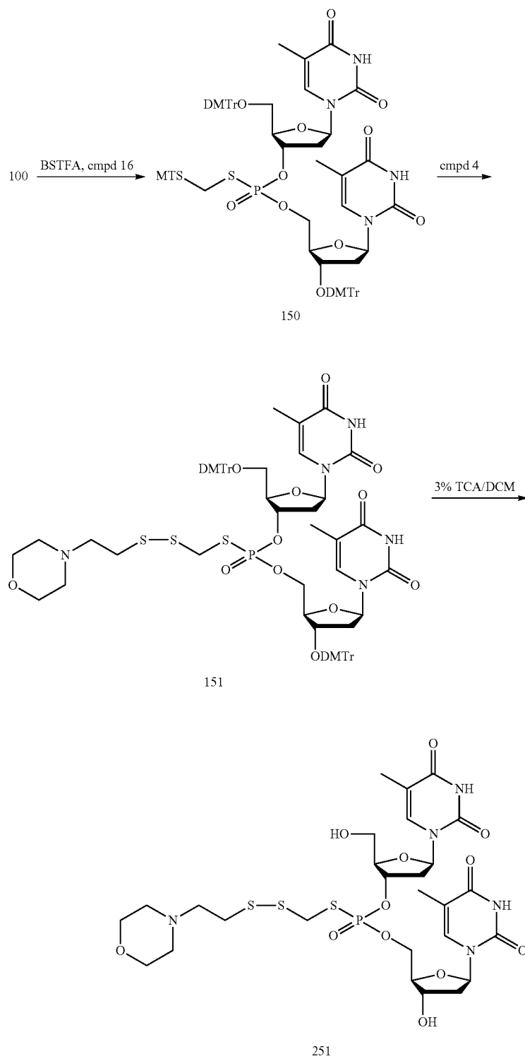
Scheme 3
