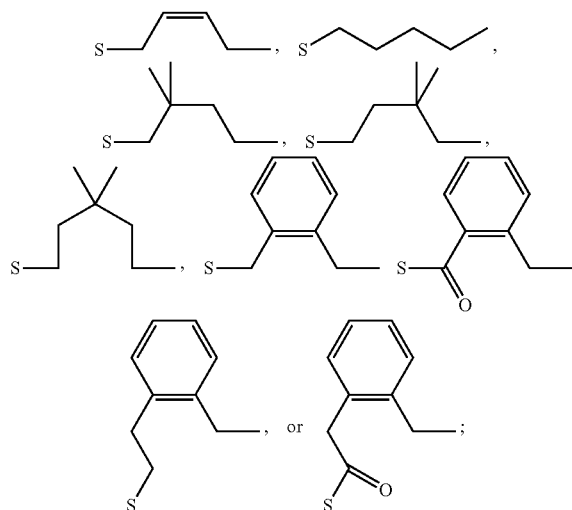
Structure IIIa
