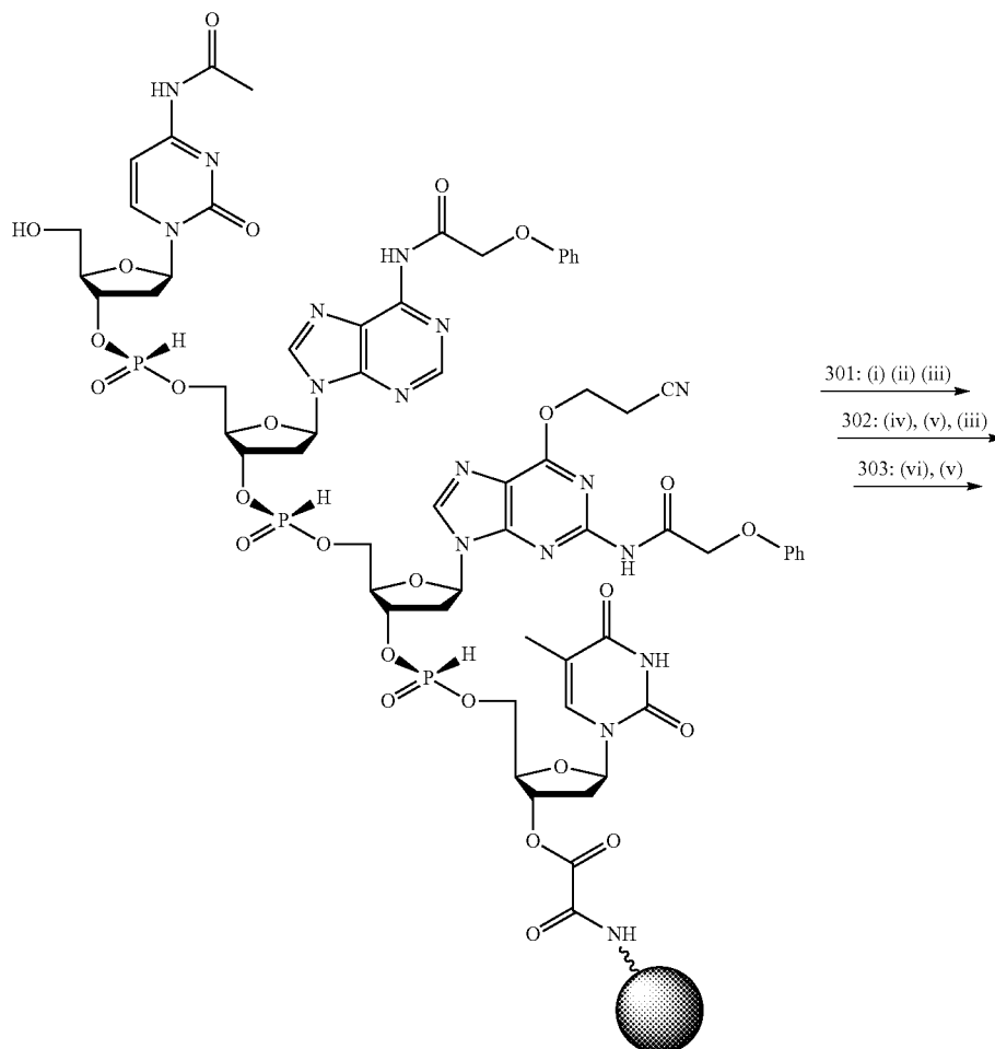
Scheme 4. Synthesis of phosphorothioate triesters on support
