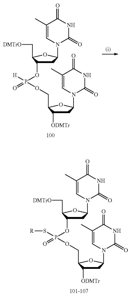
Scheme 2
