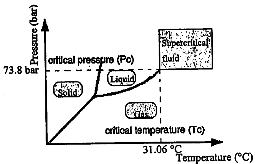
Fig 13. Pressure-temperature diagram of CO 2
