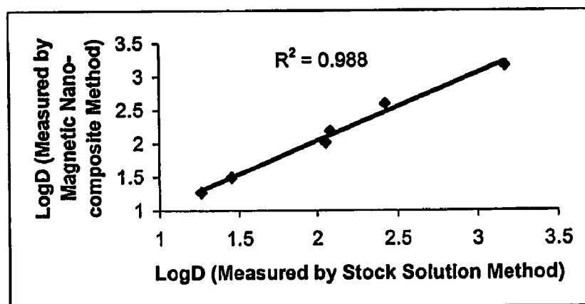
Fig 18. Correlation curve of logD values measured by using stock solution method and magnetic nano-composite method
