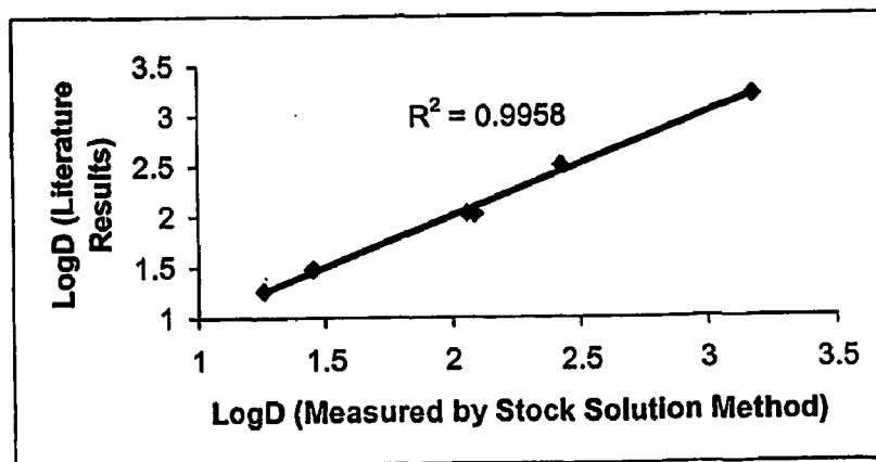
Fig 16. Correlation curve of logD values measured by using stock solution method and literature values
