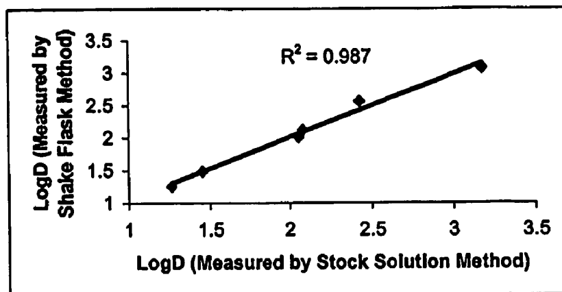
Fig 17. Correlation curve of logD values measured by using stock solution method and shake flask method
