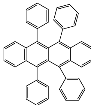
(rubrene)
