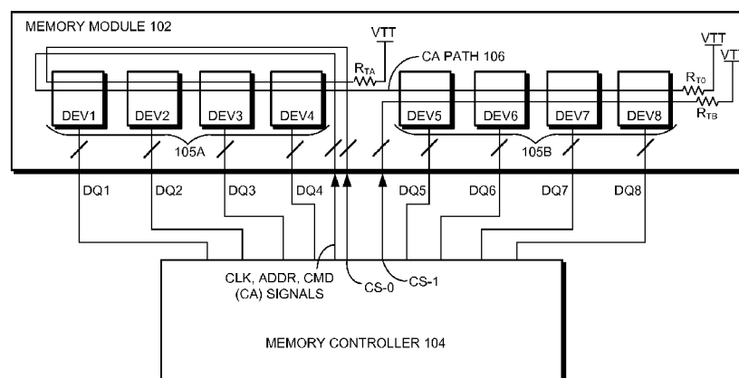
MEMORY SYSTEM 100
