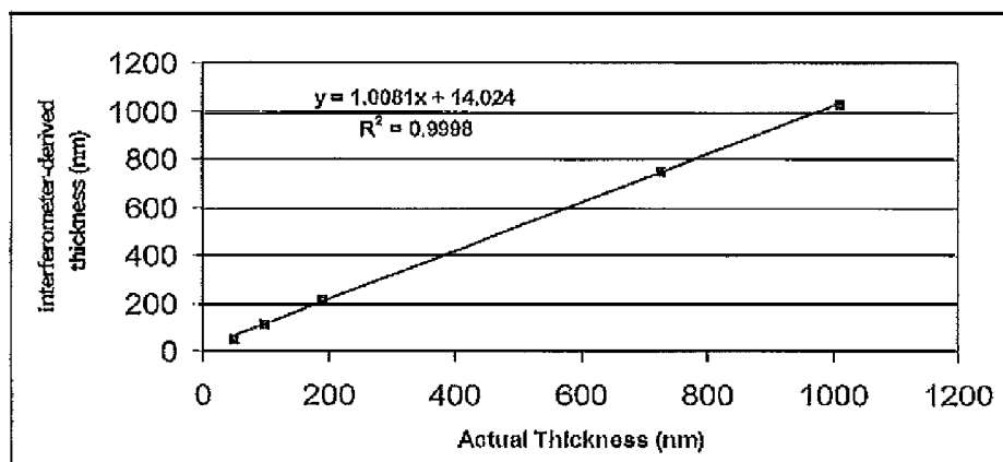
Figure 2. Standard curve from SiO 2 thin film thickness standards.
