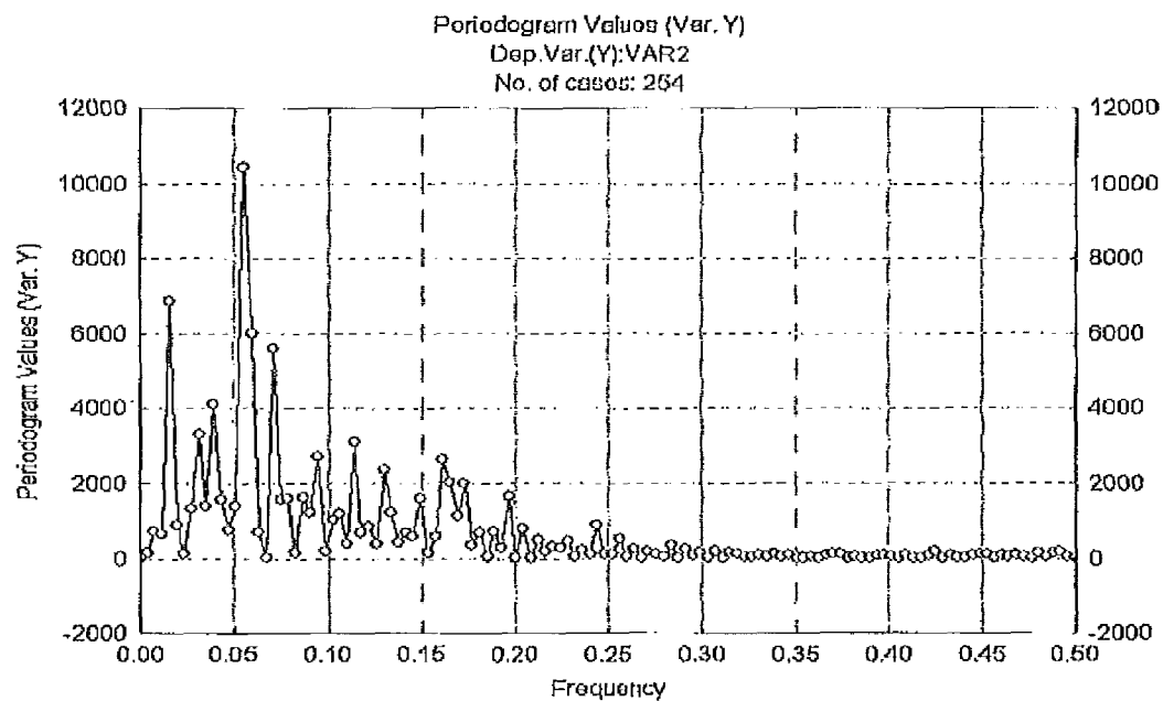
Figure 18. Fourier-Transform-frequency plot of %R vs. time plot from Figure 16.
