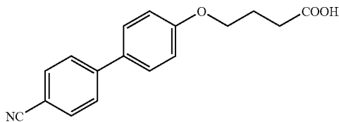
[(4'-cyano-1,1'-biphenyl-4-yl)oxy]butyric acid
