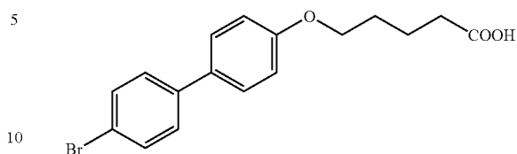
[(4'-bromo-1,1'-biphenyl-4-yl)oxy]valeric acid
