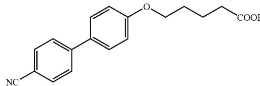
[(4'-cyano-1,1'-biphenyl-4-yl)oxy]valeric acid
