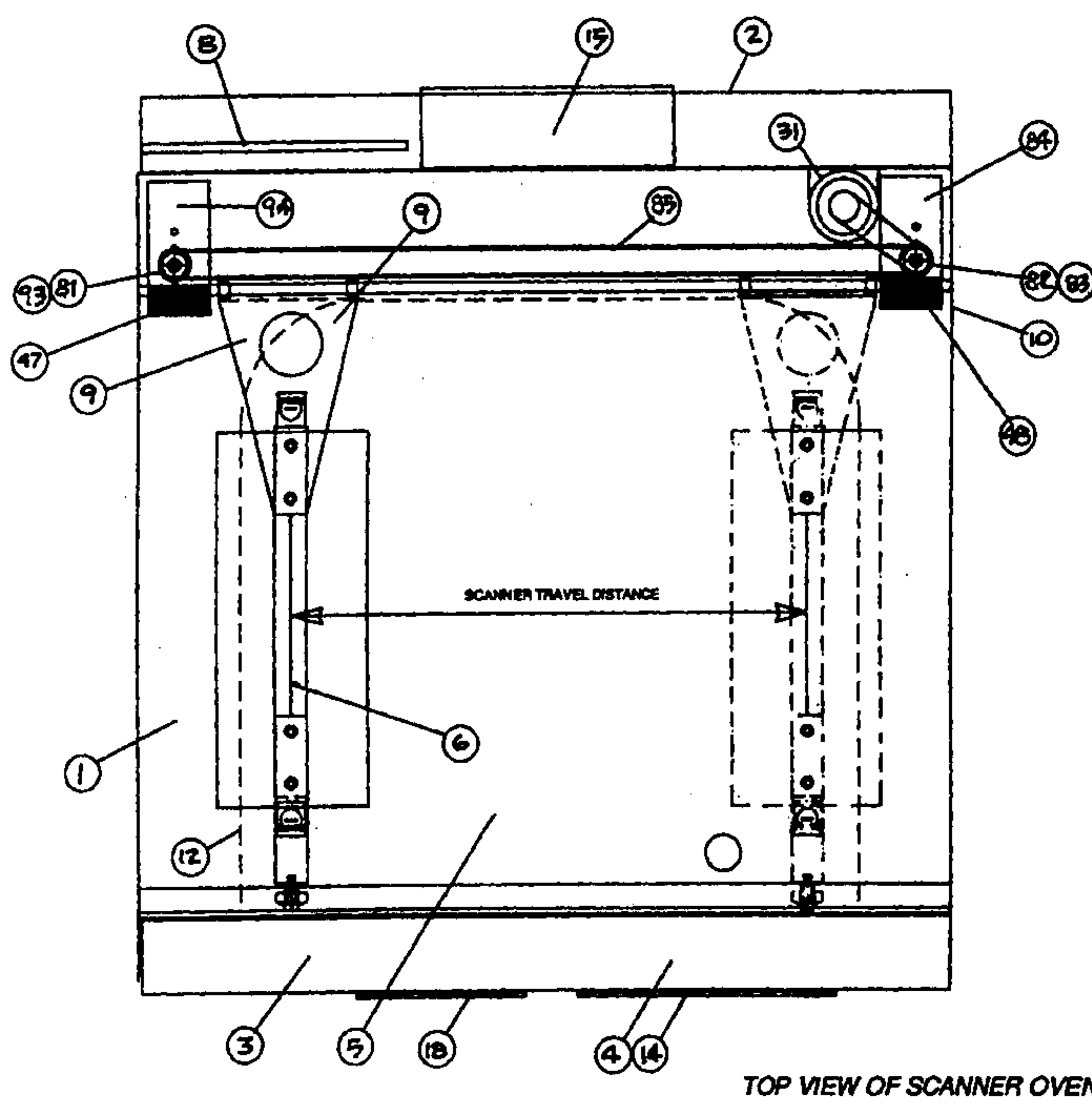
TOP VIEW OF SCANNER OVEN
