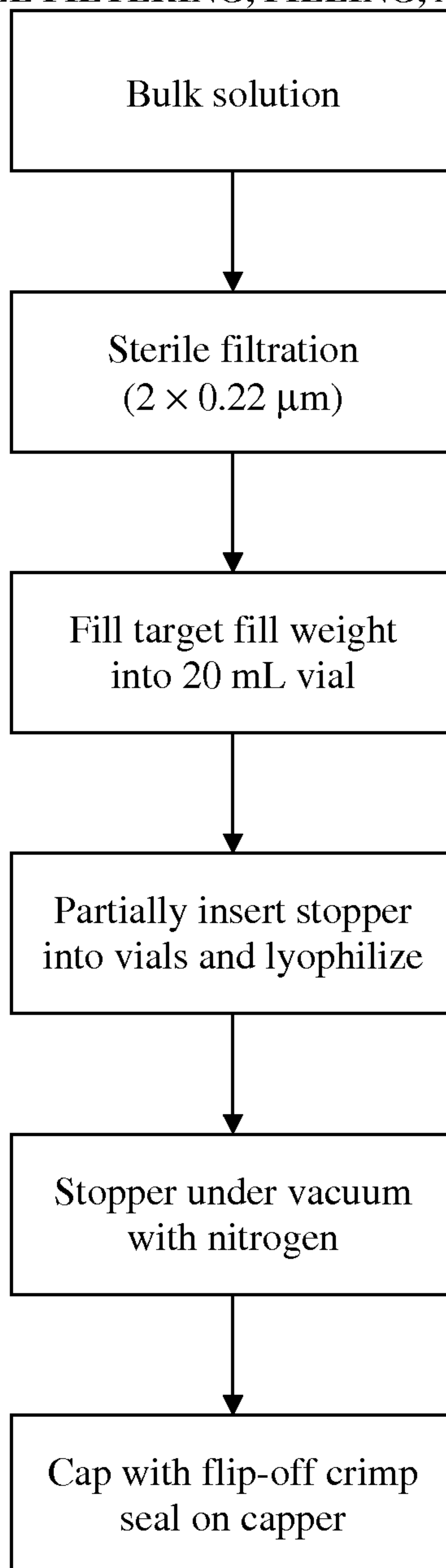
FIGURE 9 MANUFACTURING PROCESS SCHEMATIC FOR TR-701 FA FOR INJECTION, 200 MG/VIAL: STERILE FILTERING, FILLING, AND LYOPHILIZATION
