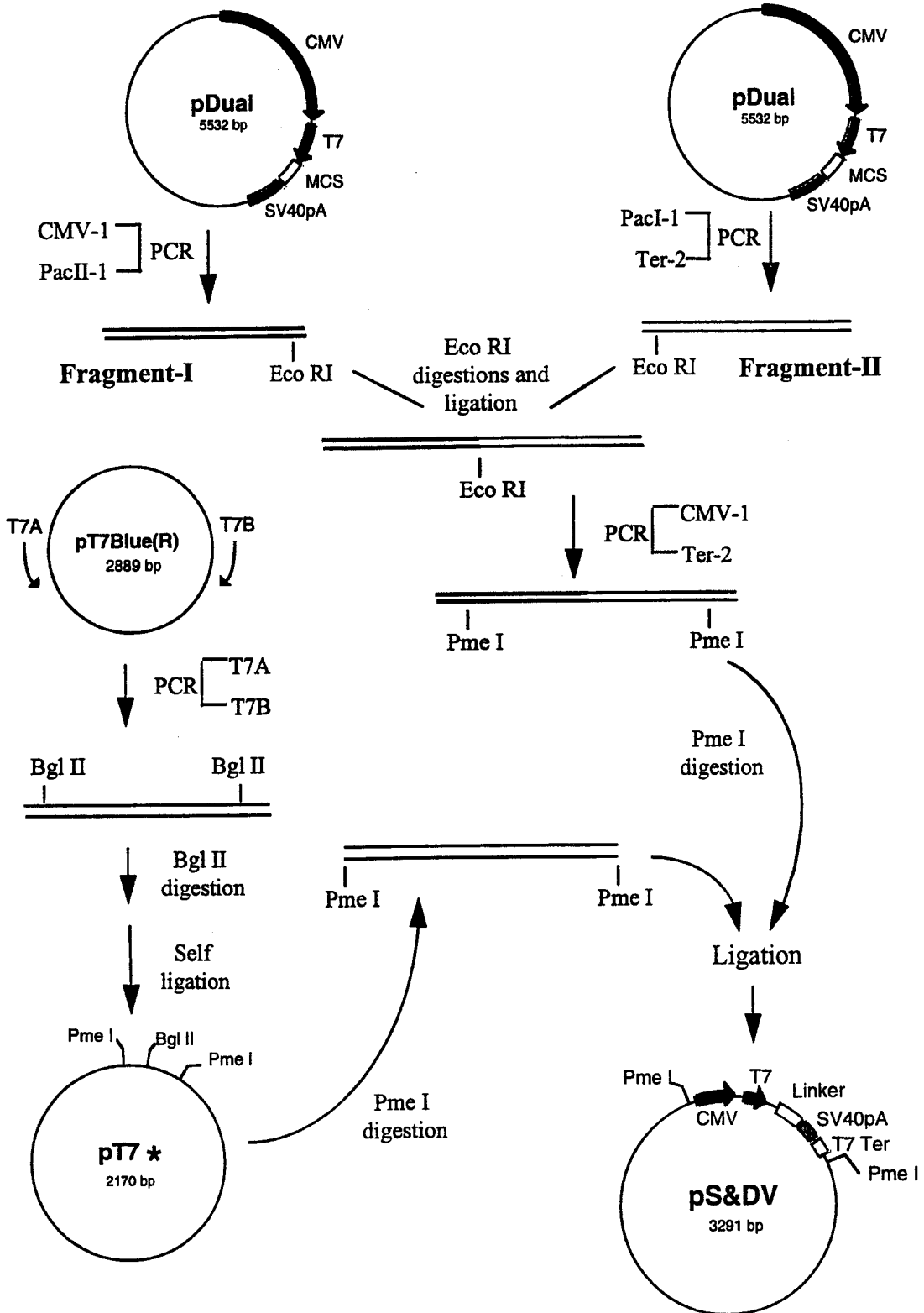
Figure 3B. Construction of Dual Expression Vector pS&DV
