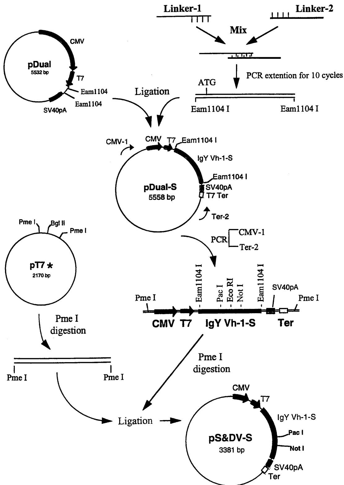
Figure 3D. Construction of Dual Expression Vector pS&DV-S
