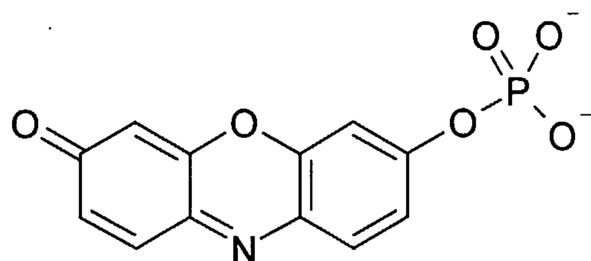
Resorufin phosphate
