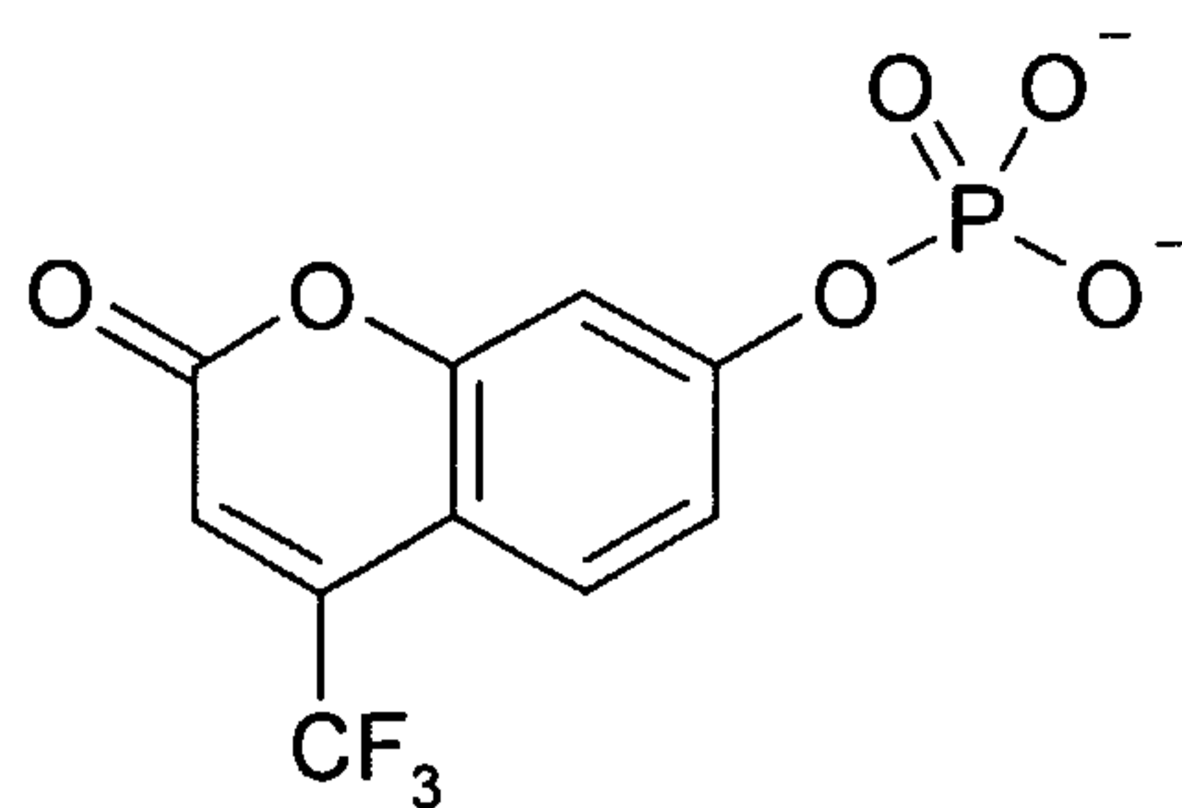
4-Trifluoromethylumbelliferyl phosphate
