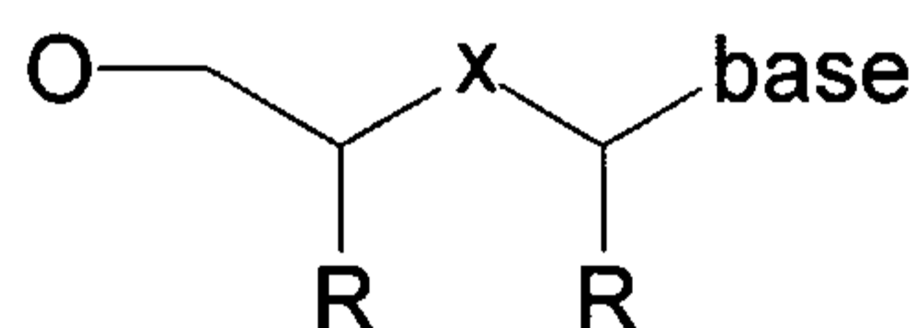
Acyclic Moieties
