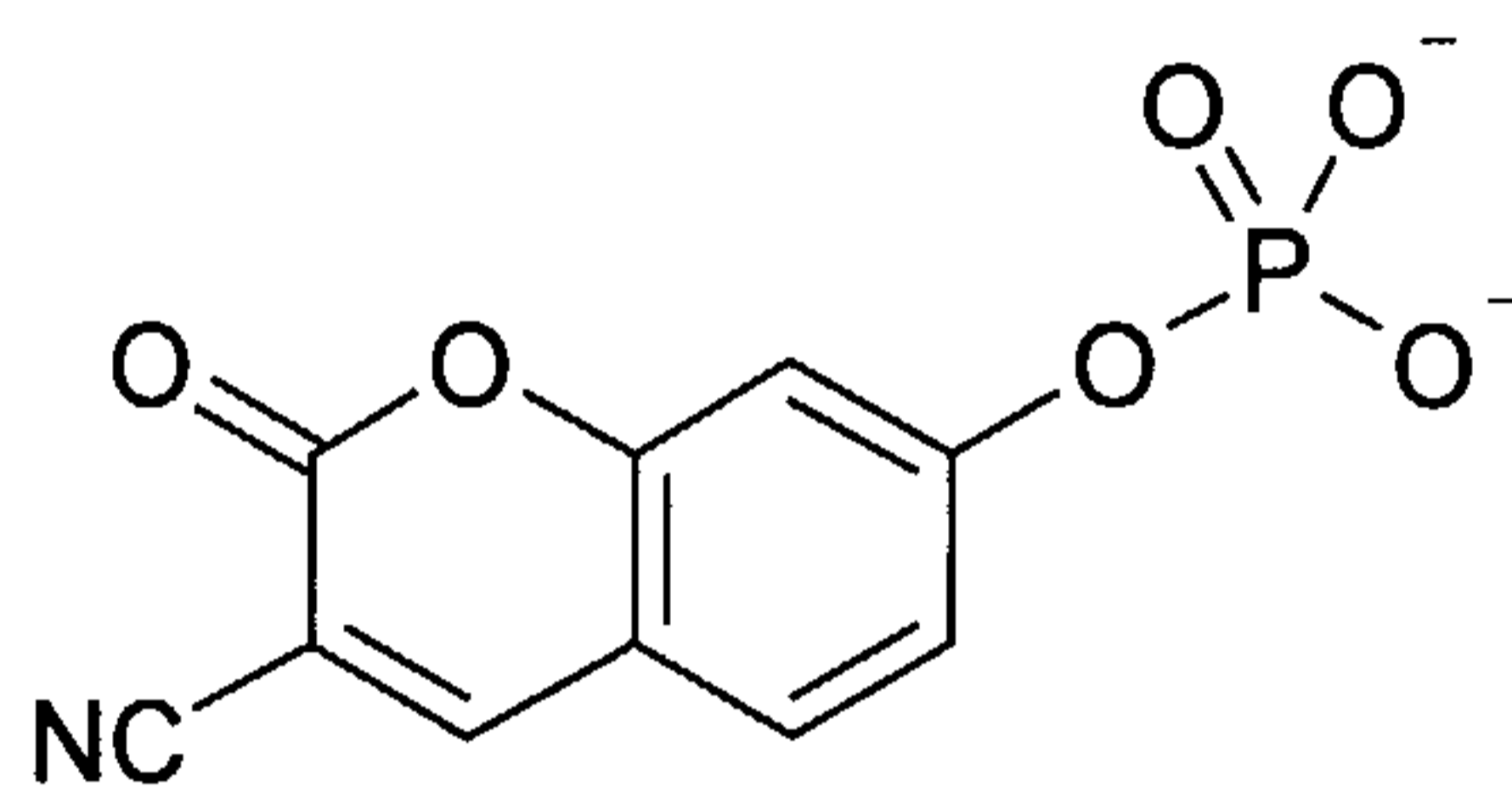
3-Cyanoumbelliferyl phosphate
