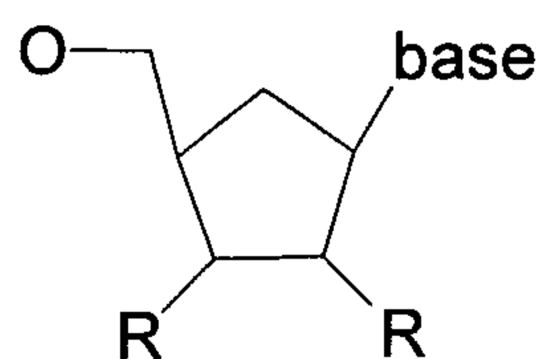
Carbocyclic Moieties
