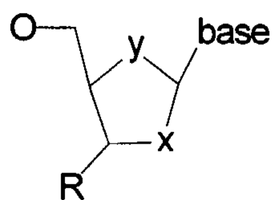
Sugar Moieties
