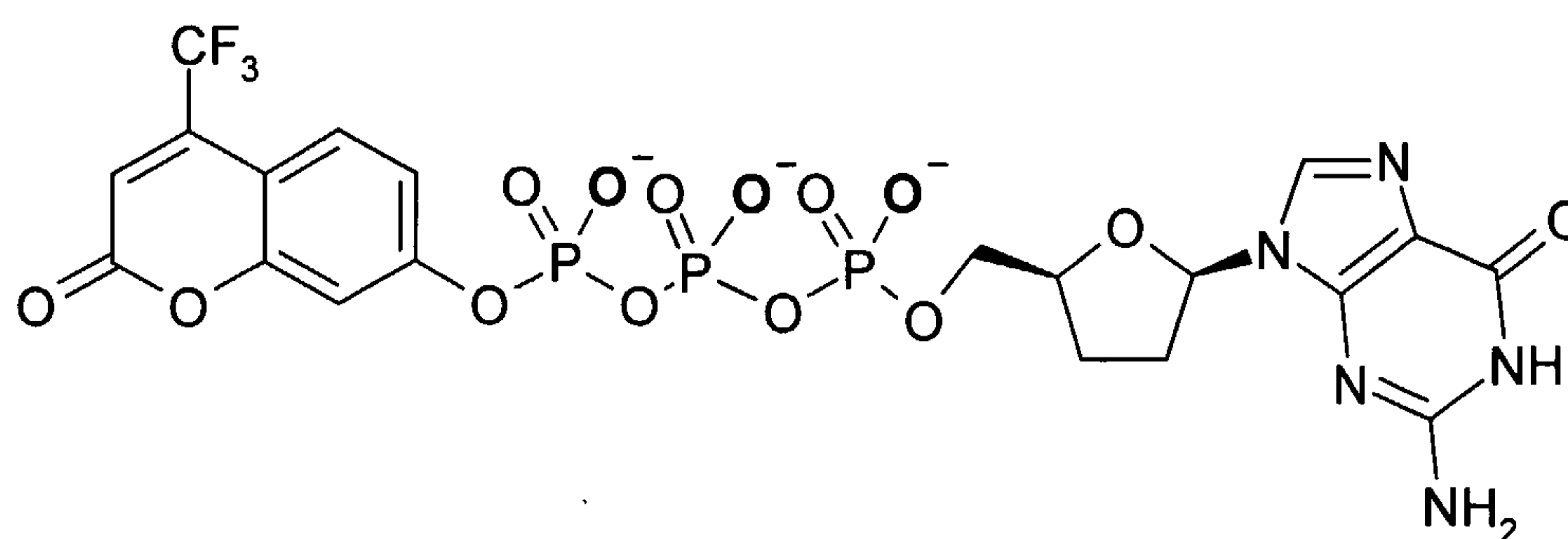
\gamma -(4-trifluoromethylcoumarinyl)dideoxyguanosine-5'-triphosphate ( \gamma CF 3 Coumarin-ddGTP)
