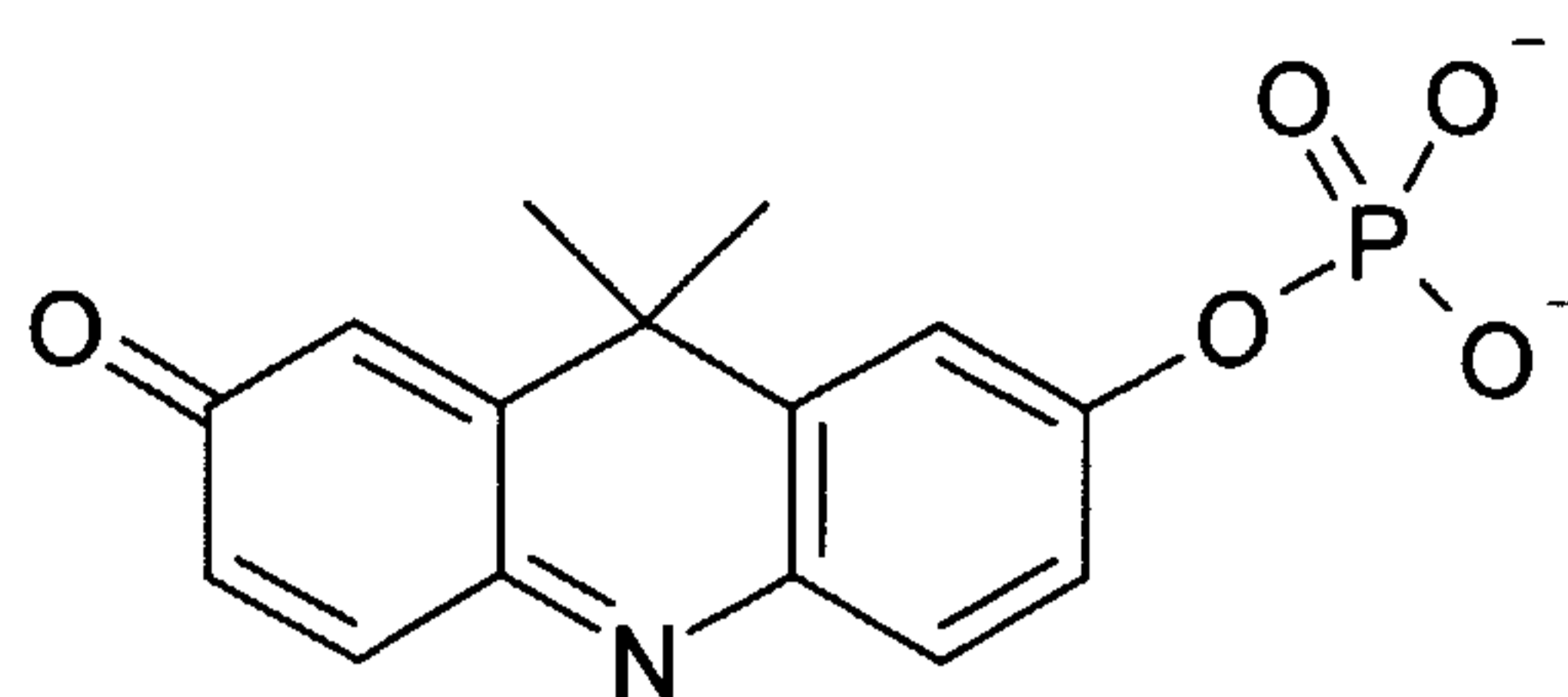
9,9-dimethylacridin-2-one-7-yl phosphate
