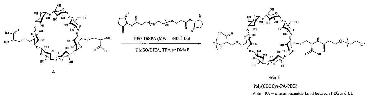
Scheme XXXVIIIa
