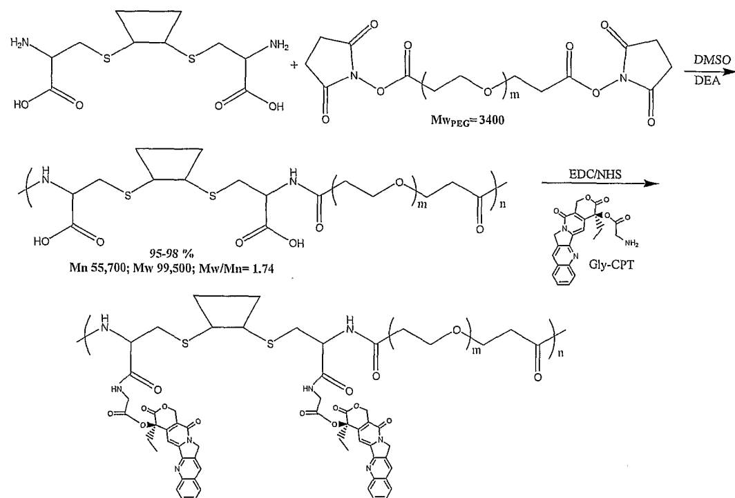
Scheme XIII
