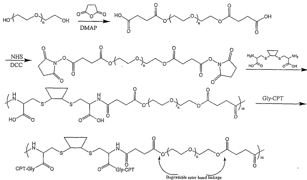
5 Scheme XIV
