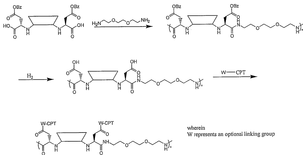
Scheme IV
