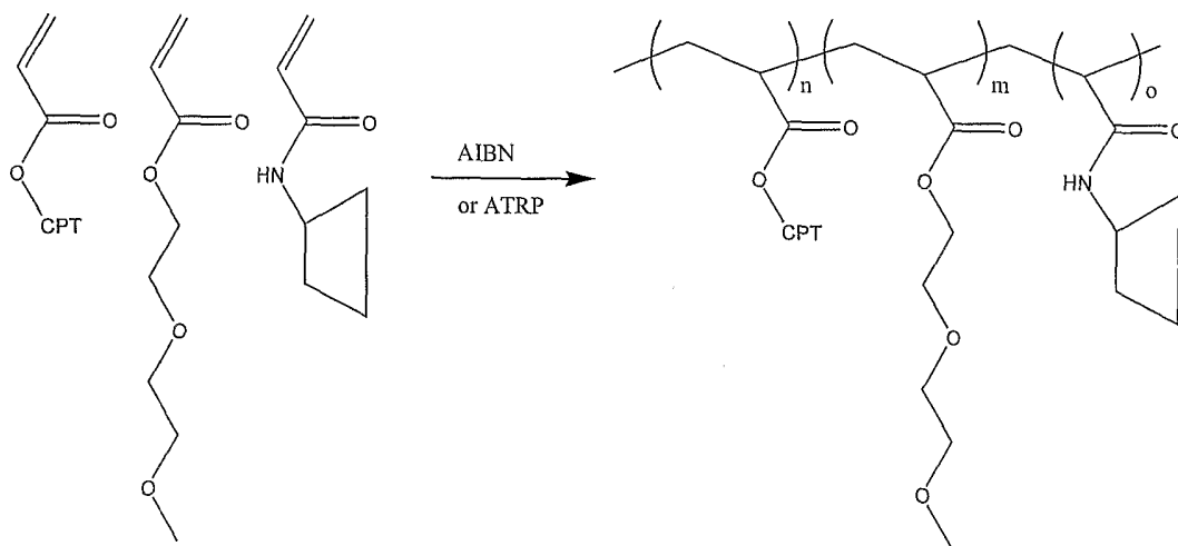
Scheme X
