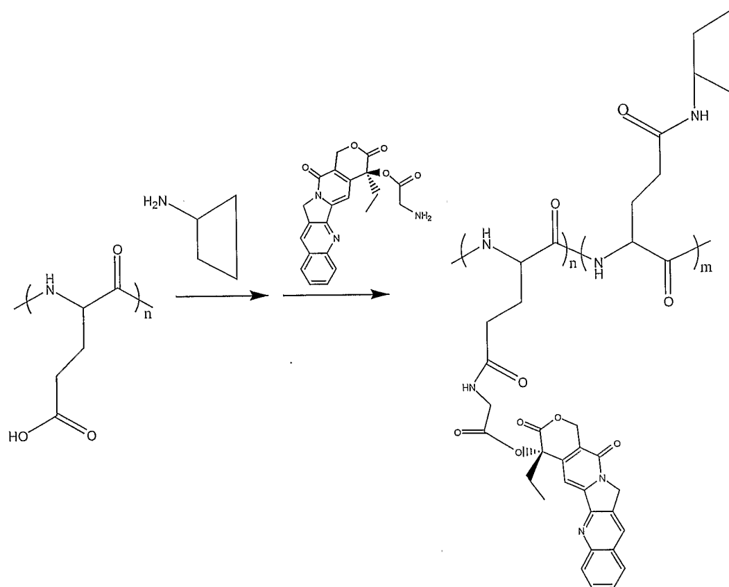
Scheme XII
