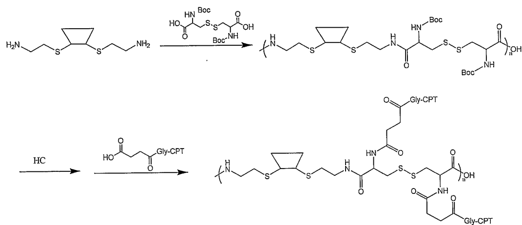
Scheme VII
