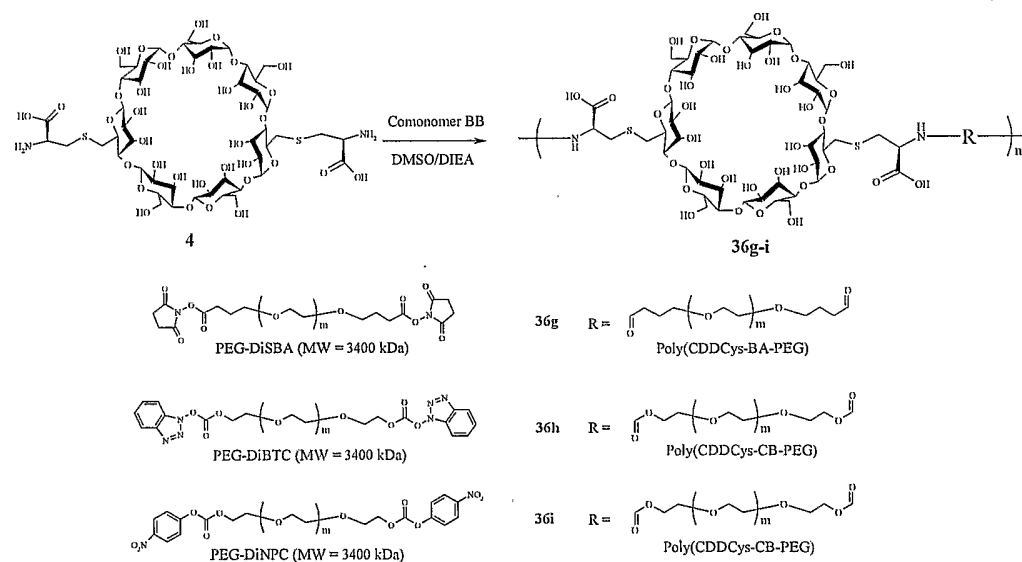
Scheme XXXVIIIb
