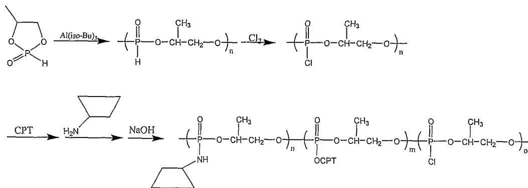
Scheme IX
