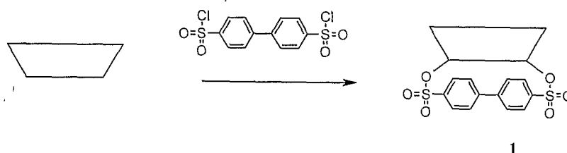
Scheme XV
