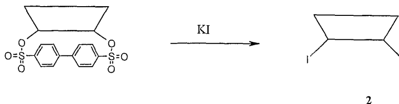
Scheme XVI
