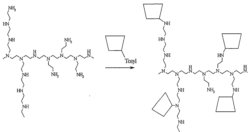
Scheme XXXXIV
