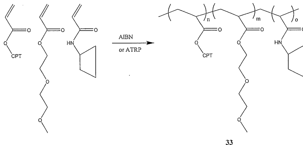
Scheme XXXV
