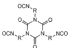
cyanurate trimer
