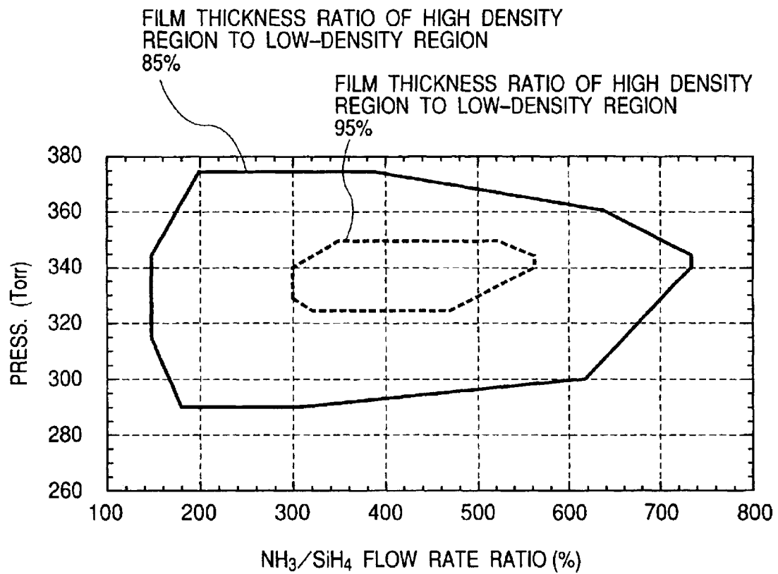
FIG. 3 REGIONS OF AN NH 3 /SiH 4 FLOW RATE RATIO AND A FILM FORMING PRESSURE PERMITTING A FILM THICKNESS RATIO OF HIGH DENSITY REGION TO LOW-DENSITY REGION NOT LESS THAN 85% AND NOT LESS THAN 95%
