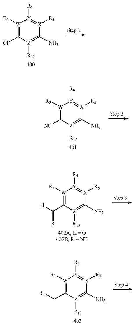
Reaction Scheme 4
