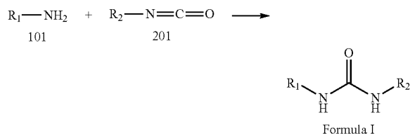
REACTION SCHEME 2
