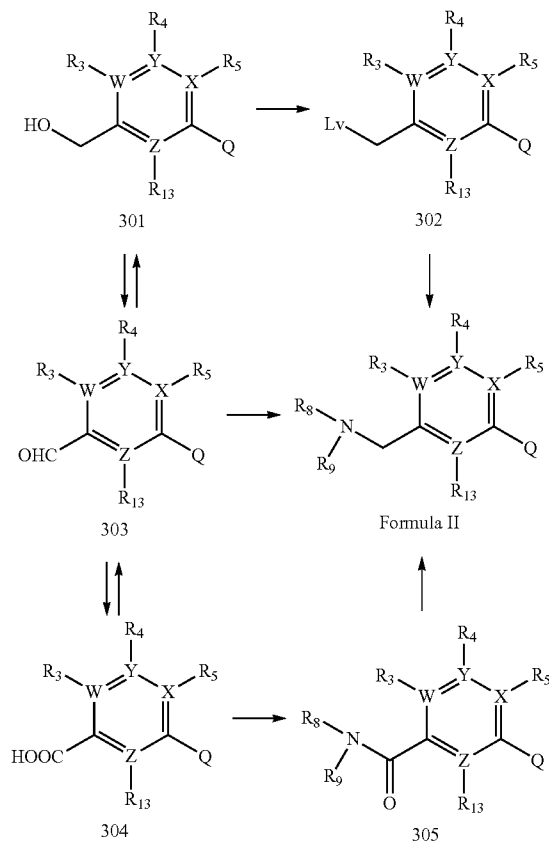
REACTION SCHEME 3
