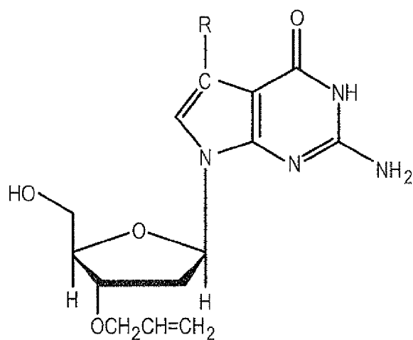
G-42; \text{R}=\text{CCCH}_2\text{NHCOCF}_3
