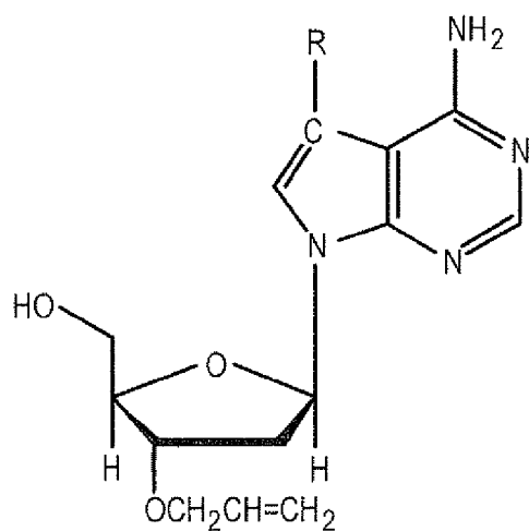
A-37; \text{R}=\text{CCCH}_2\text{NHCOCF}_3
