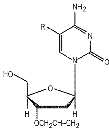
C-21; \text{R}=\text{CCCH}_2\text{NHCOCF}_3
