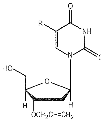
U-26; \text{R}=\text{CCCH}_2\text{NHCOCF}_3
