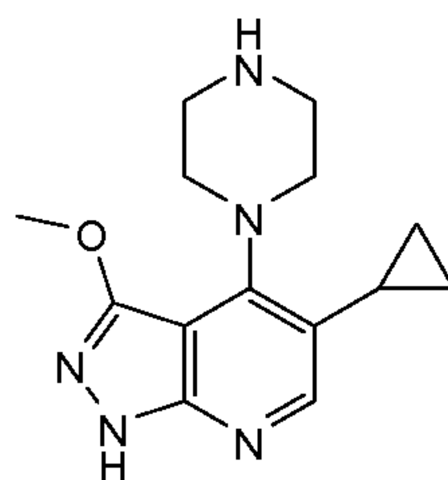
5-cyclopropyl-3-methoxy-4-(piperazin-1-yl)-1H-pyrazolo[3,4-b]pyridine
