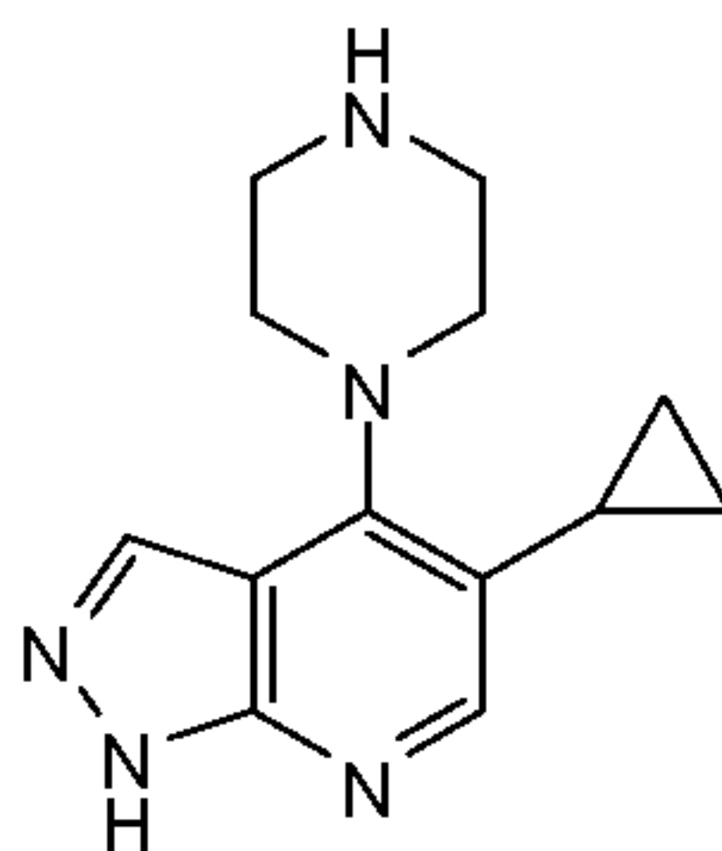
5-cyclopropyl-4-(piperazin-1-yl)-1H-pyrazolo[3,4-b]pyridine
