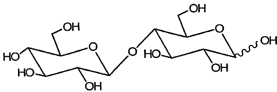
FIG. 5 Structure of Cellobiose
