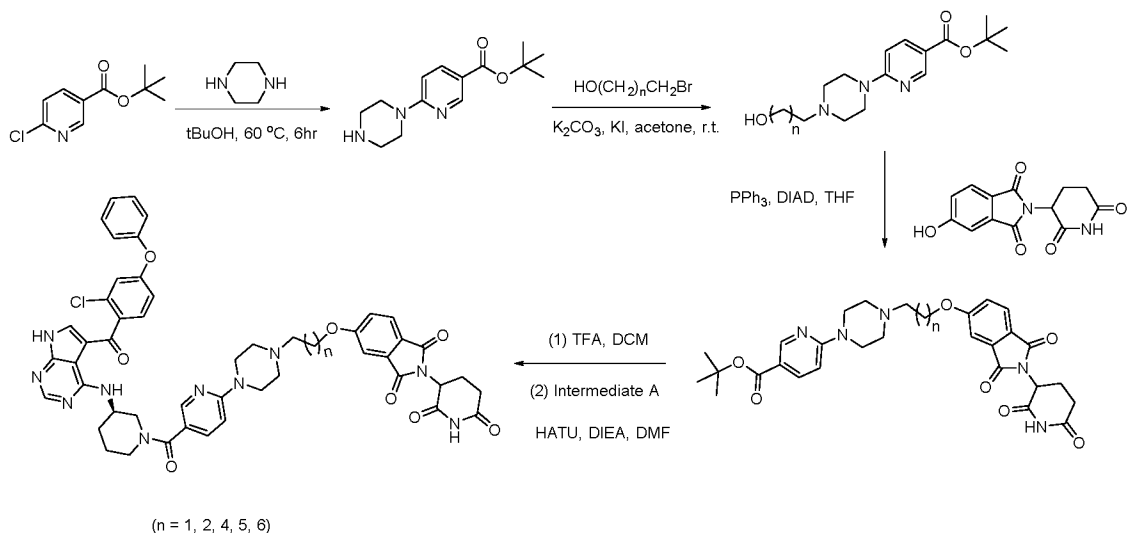
Scheme 2: Method for the preparation of compound 2
