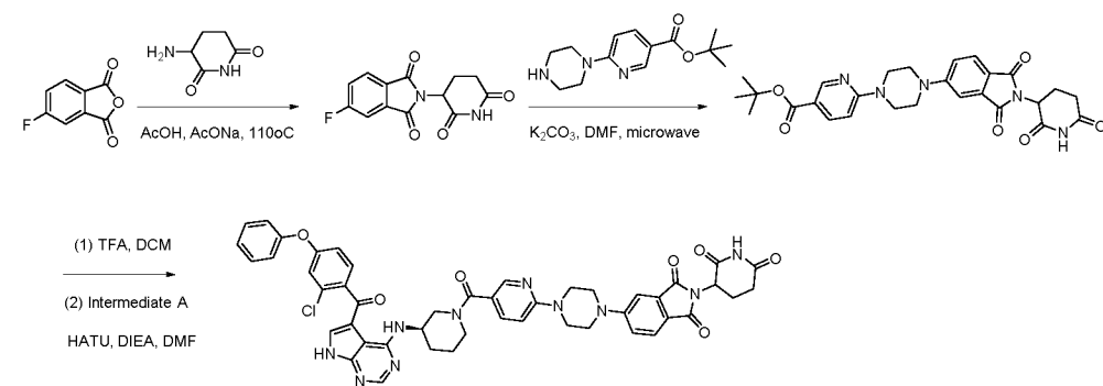
Scheme 3: Method for the preparation of compounds 7, 8, 11, and 19
