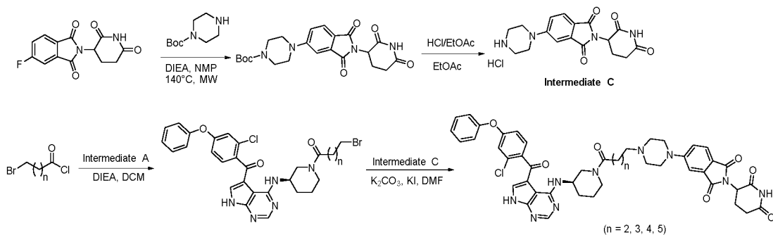
Scheme 3: Method for the preparation of compounds 7, 8, 11, and 19
