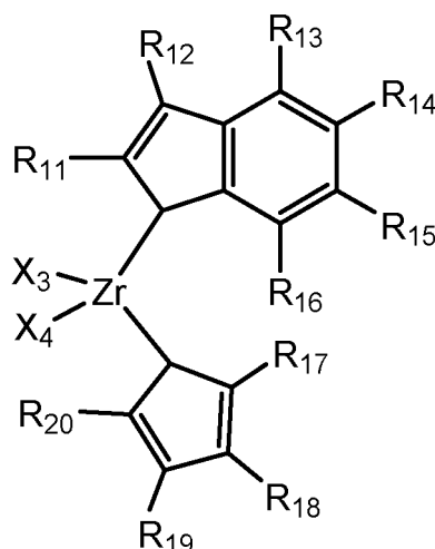
[Chemical Formula 2]
