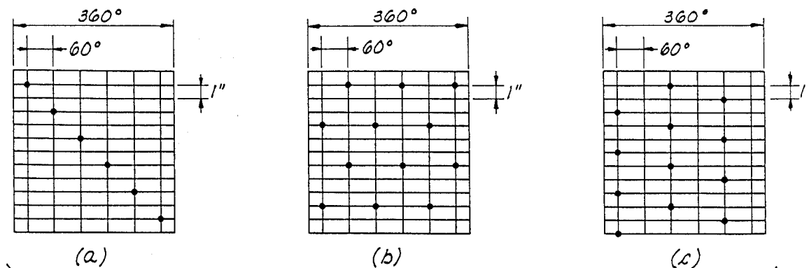
FIG. 1 PRIOR ART
